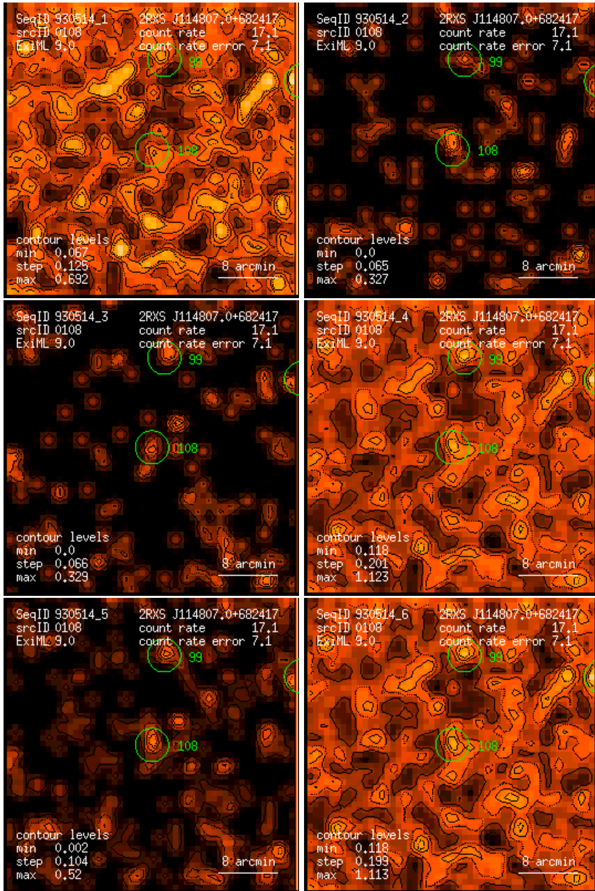
Figure 108: RASS 930514: detection 0108: band rate images, Gaussian filter: (1) PSPC channels 11 – 41, (2) 52 – 90, (3) 91 – 201, (4) 11 – 235, (5) 52 – 201, (6) 11 – 201. Broad band rates in counts/ks. Band rate contour levels in counts/ks/arcmin 2 .
