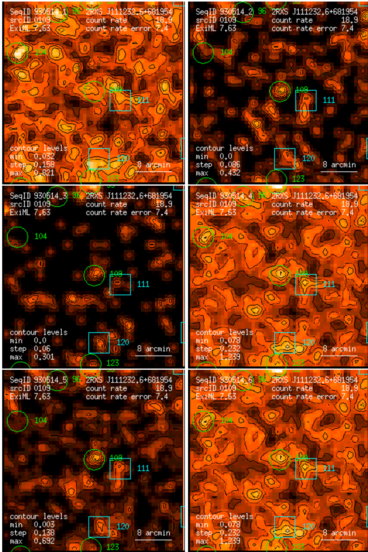
Figure 109: RASS 930514: detection 0109: band rate images, Gaussian filter: (1) PSPC channels 11 – 41, (2) 52 – 90, (3) 91 – 201, (4) 11 – 235, (5) 52 – 201, (6) 11 – 201. Broad band rates in counts/ks. Band rate contour levels in counts/ks/arcmin 2 .
