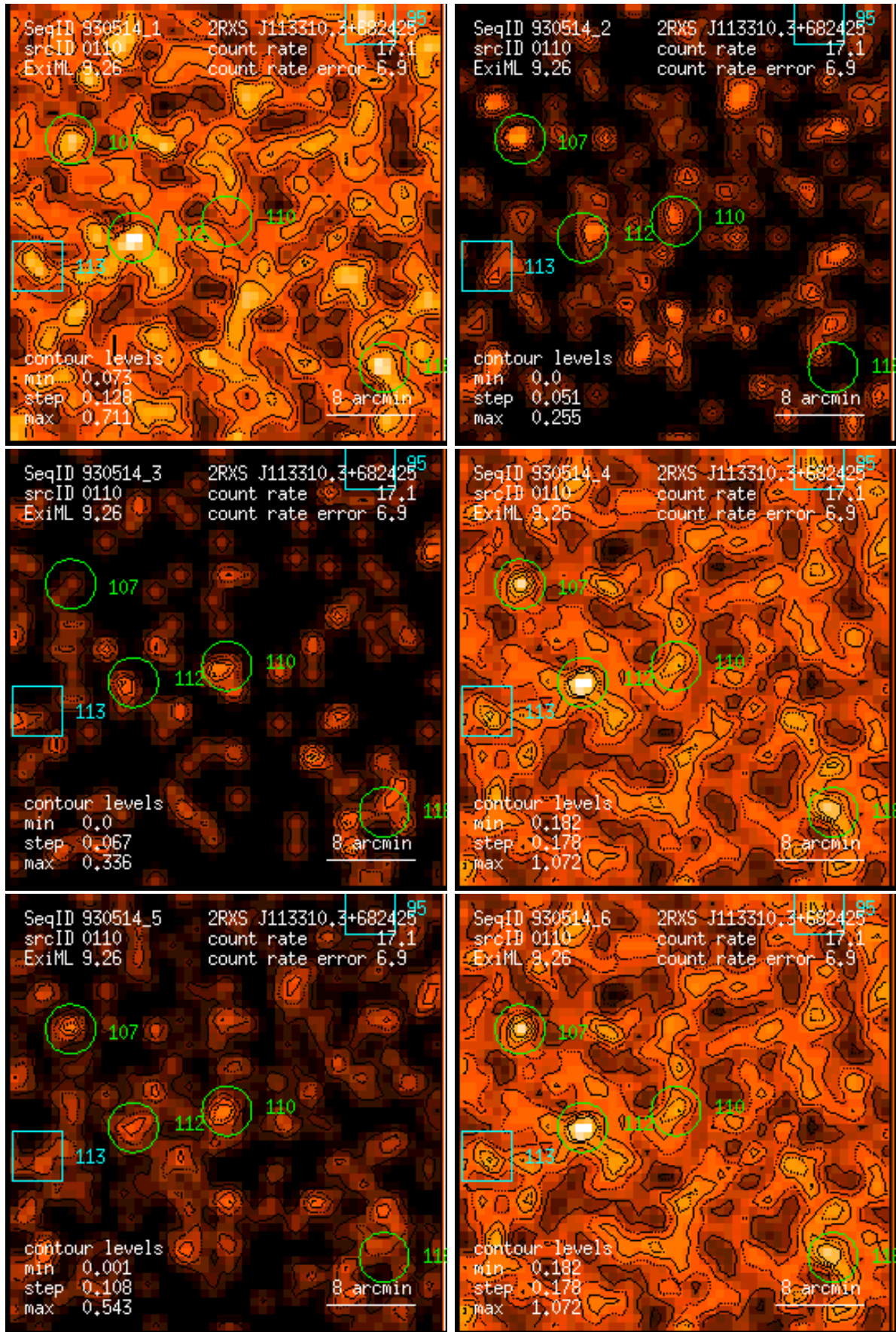
Figure 110: RASS 930514: detection 0110: band rate images, Gaussian filter: (1) PSPC channels 11 – 41, (2) 52 – 90, (3) 91 – 201, (4) 11 – 235, (5) 52 – 201, (6) 11 – 201. Broad band rates in counts/ks. Band rate contour levels in counts/ks/arcmin 2 .
