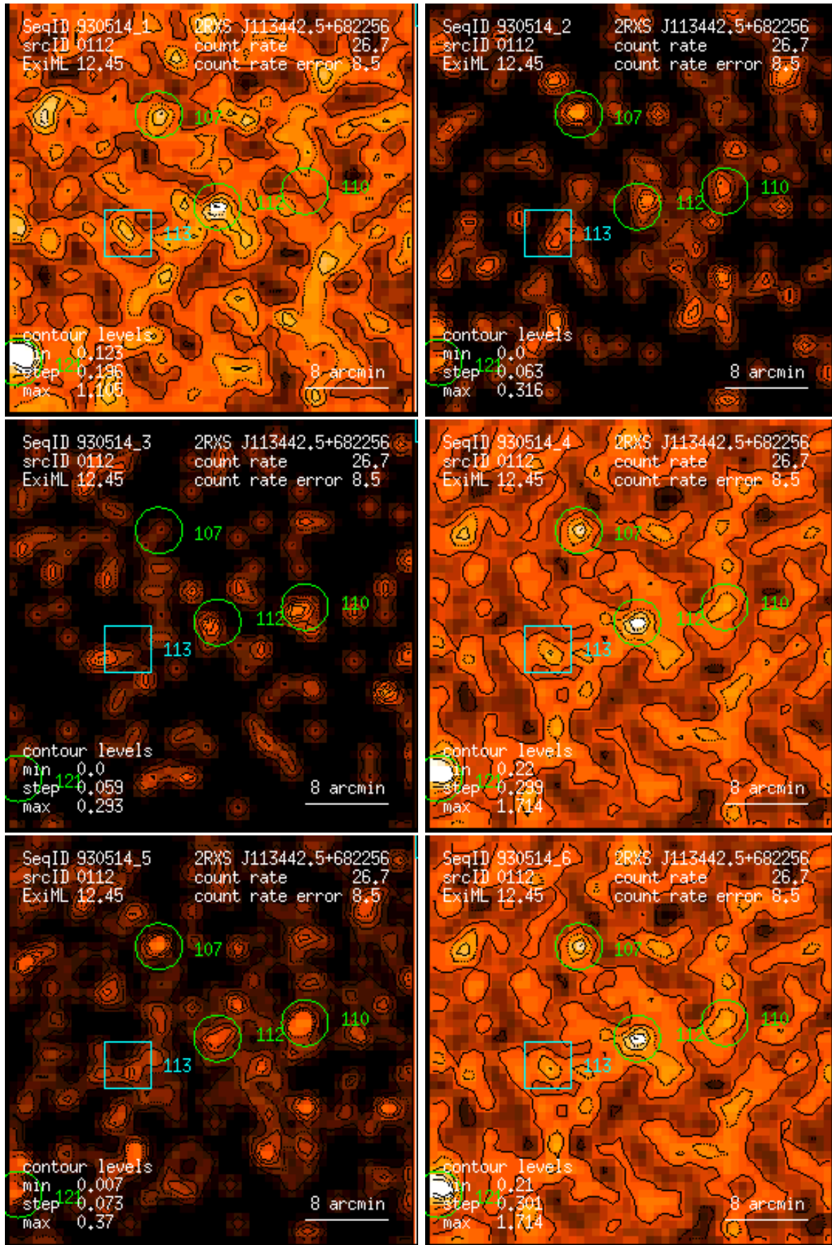
Figure 112: RASS 930514: detection 0112: band rate images, Gaussian filter: (1) PSPC channels 11 – 41, (2) 52 – 90, (3) 91 – 201, (4) 11 – 235, (5) 52 – 201, (6) 11 – 201. Broad band rates in counts/ks. Band rate contour levels in counts/ks/arcmin 2 .
