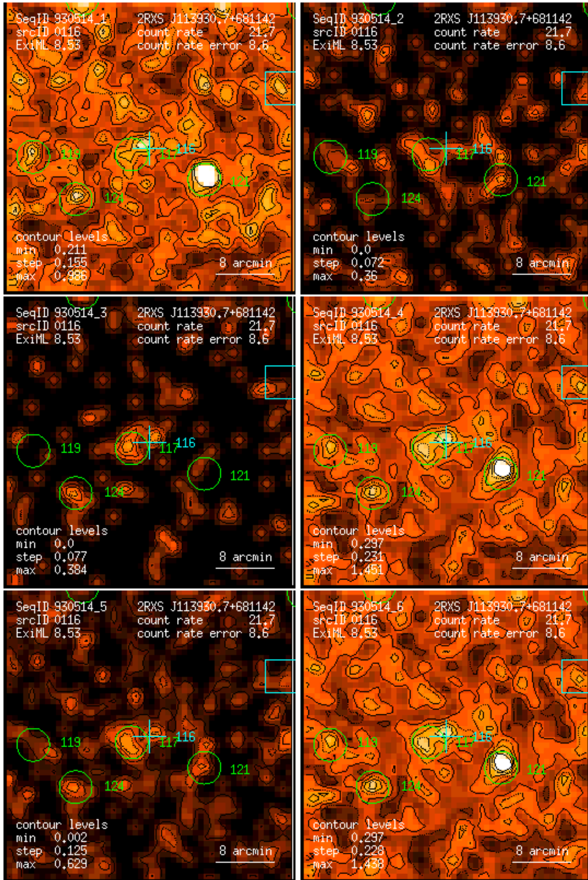
Figure 116: RASS 930514: detection 0116: band rate images, Gaussian filter: (1) PSPC channels 11 – 41, (2) 52 – 90, (3) 91 – 201, (4) 11 – 235, (5) 52 – 201, (6) 11 – 201. Broad band rates in counts/ks. Band rate contour levels in counts/ks/arcmin 2 .
