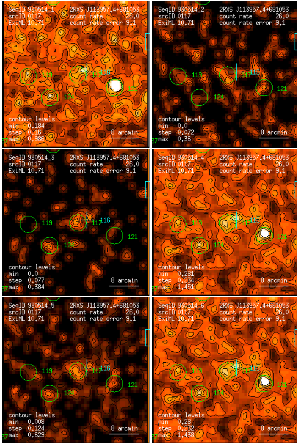
Figure 117: RASS 930514: detection 0117: band rate images, Gaussian filter: (1) PSPC channels 11 – 41, (2) 52 – 90, (3) 91 – 201, (4) 11 – 235, (5) 52 – 201, (6) 11 – 201. Broad band rates in counts/ks. Band rate contour levels in counts/ks/arcmin 2 .
