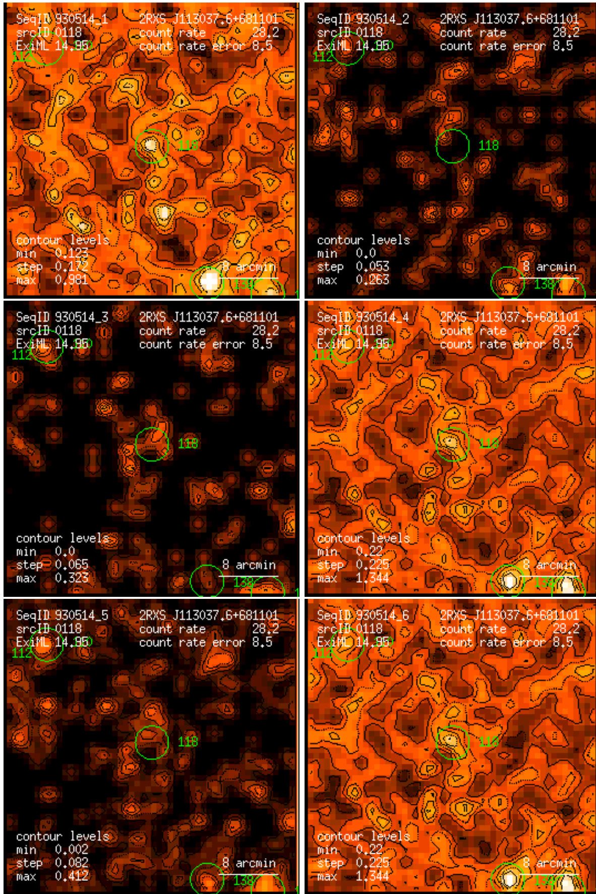
Figure 118: RASS 930514: detection 0118: band rate images, Gaussian filter: (1) PSPC channels 11 – 41, (2) 52 – 90, (3) 91 – 201, (4) 11 – 235, (5) 52 – 201, (6) 11 – 201. Broad band rates in counts/ks. Band rate contour levels in counts/ks/arcmin 2 .
