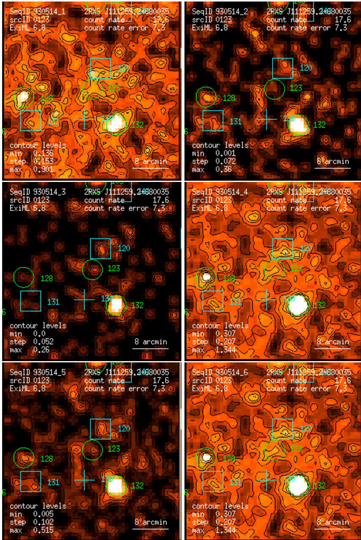
Figure 123: RASS 930514: detection 0123: band rate images, Gaussian filter: (1) PSPC channels 11 – 41, (2) 52 – 90, (3) 91 – 201, (4) 11 – 235, (5) 52 – 201, (6) 11 – 201. Broad band rates in counts/ks. Band rate contour levels in counts/ks/arcmin 2 .
