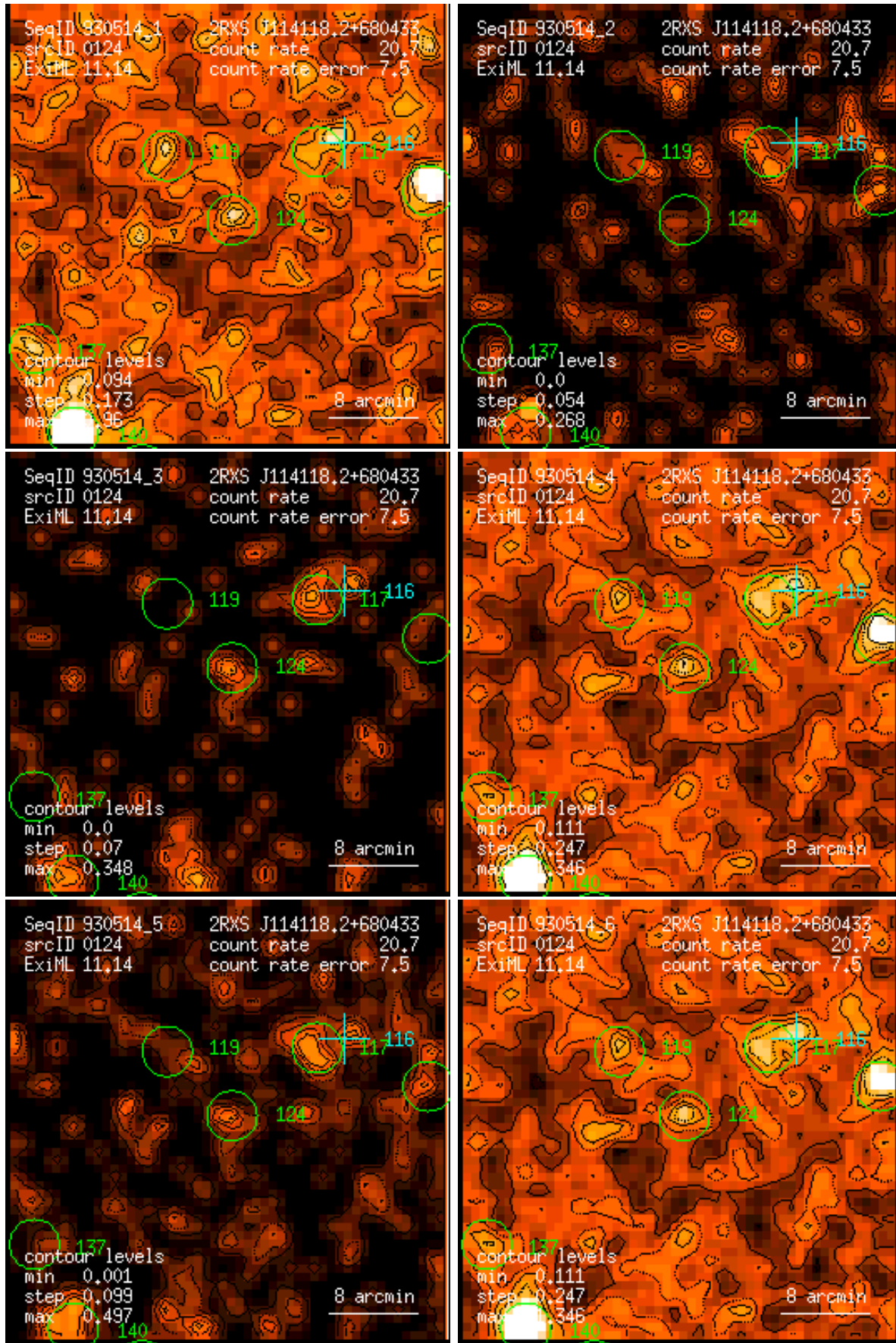
Figure 124: RASS 930514: detection 0124: band rate images, Gaussian filter: (1) PSPC channels 11 – 41, (2) 52 – 90, (3) 91 – 201, (4) 11 – 235, (5) 52 – 201, (6) 11 – 201. Broad band rates in counts/ks. Band rate contour levels in counts/ks/arcmin 2 .
