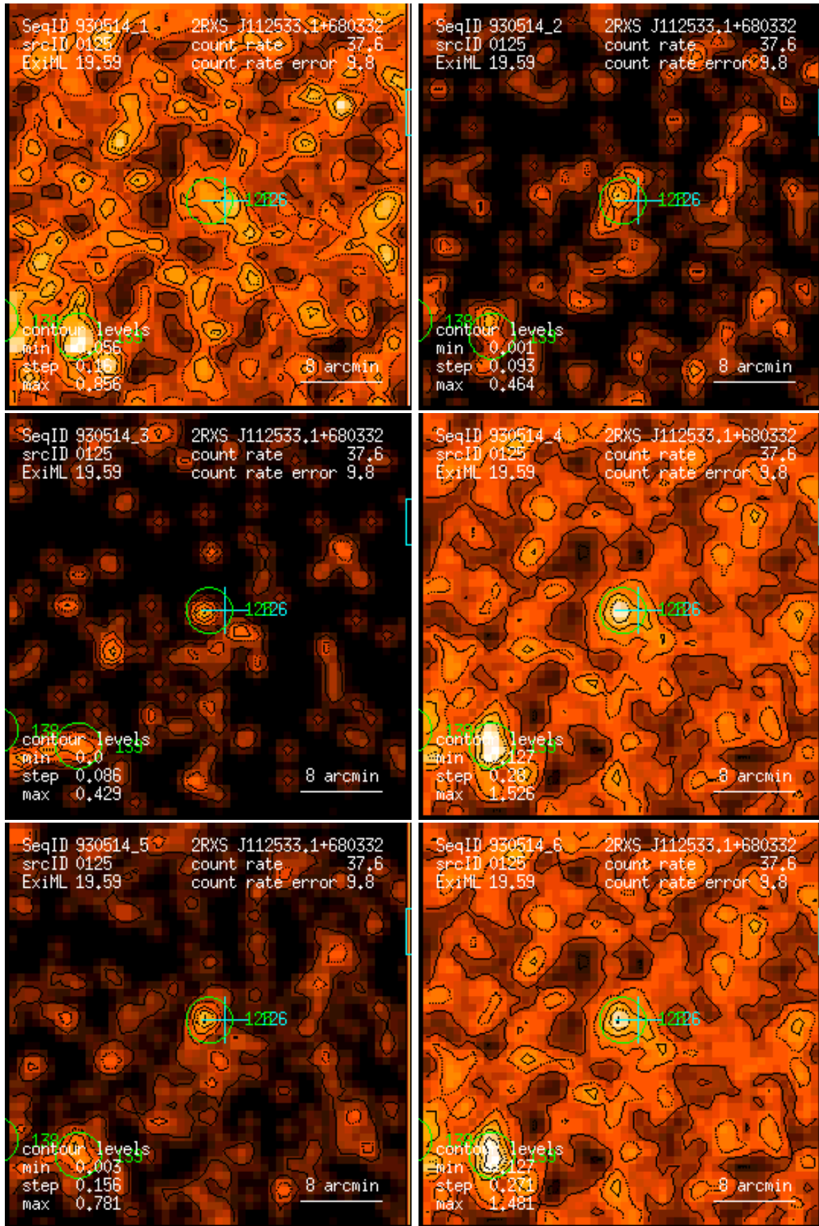
Figure 125: RASS 930514: detection 0125: band rate images, Gaussian filter: (1) PSPC channels 11 – 41, (2) 52 – 90, (3) 91 – 201, (4) 11 – 235, (5) 52 – 201, (6) 11 – 201. Broad band rates in counts/ks. Band rate contour levels in counts/ks/arcmin 2 .
