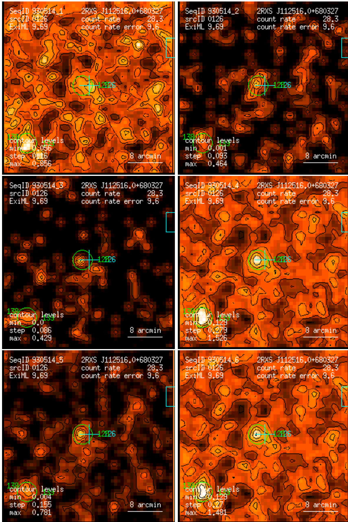
Figure 126: RASS 930514: detection 0126: band rate images, Gaussian filter: (1) PSPC channels 11 – 41, (2) 52 – 90, (3) 91 – 201, (4) 11 – 235, (5) 52 – 201, (6) 11 – 201. Broad band rates in counts/ks. Band rate contour levels in counts/ks/arcmin 2 .
