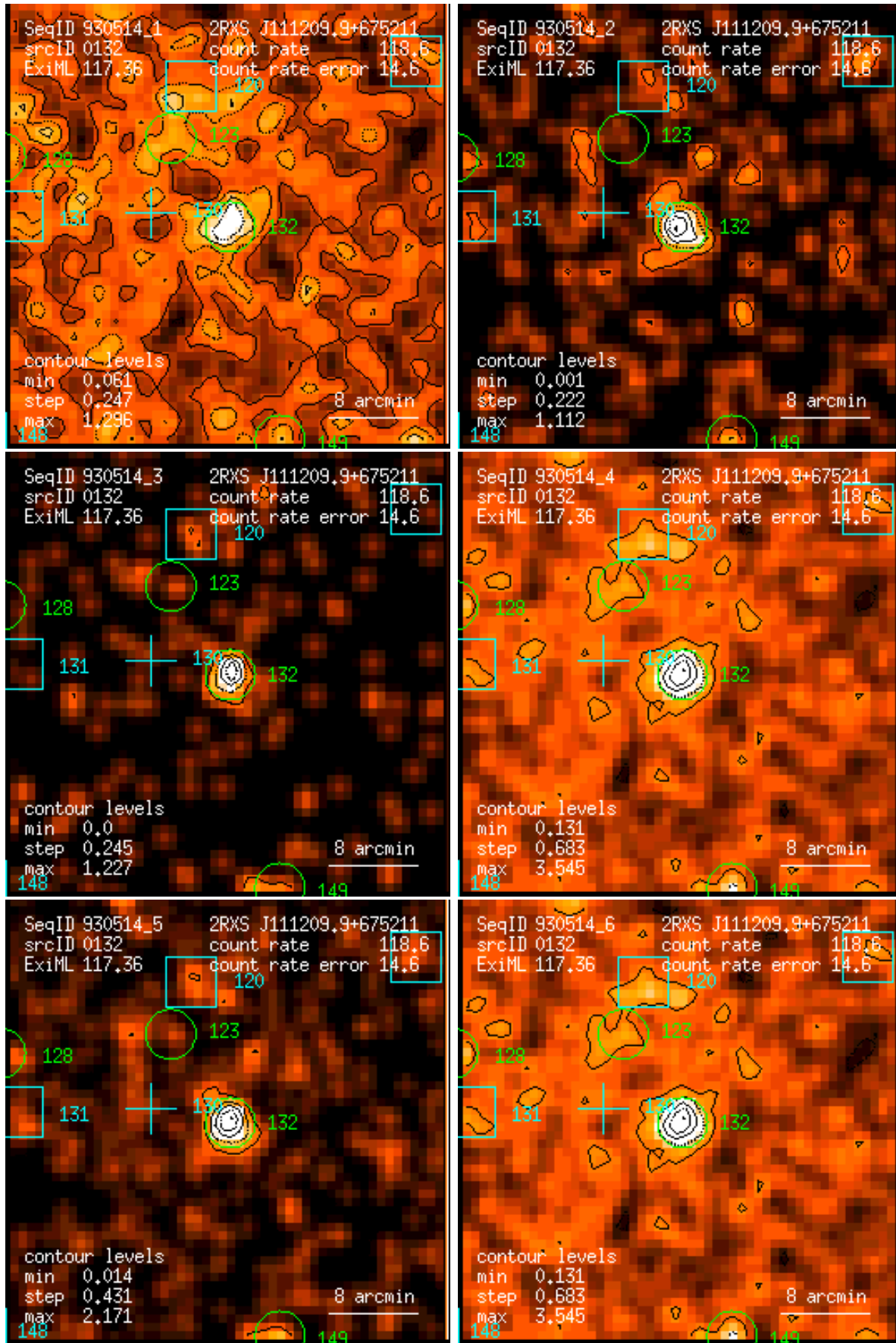
Figure 132: RASS 930514: detection 0132: band rate images, Gaussian filter: (1) PSPC channels 11 – 41, (2) 52 – 90, (3) 91 – 201, (4) 11 – 235, (5) 52 – 201, (6) 11 – 201. Broad band rates in counts/ks. Band rate contour levels in counts/ks/arcmin 2 .
