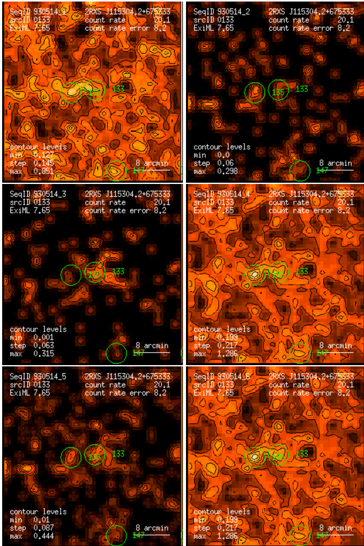
Figure 133: RASS 930514: detection 0133: band rate images, Gaussian filter: (1) PSPC channels 11 – 41, (2) 52 – 90, (3) 91 – 201, (4) 11 – 235, (5) 52 – 201, (6) 11 – 201. Broad band rates in counts/ks. Band rate contour levels in counts/ks/arcmin 2 .
