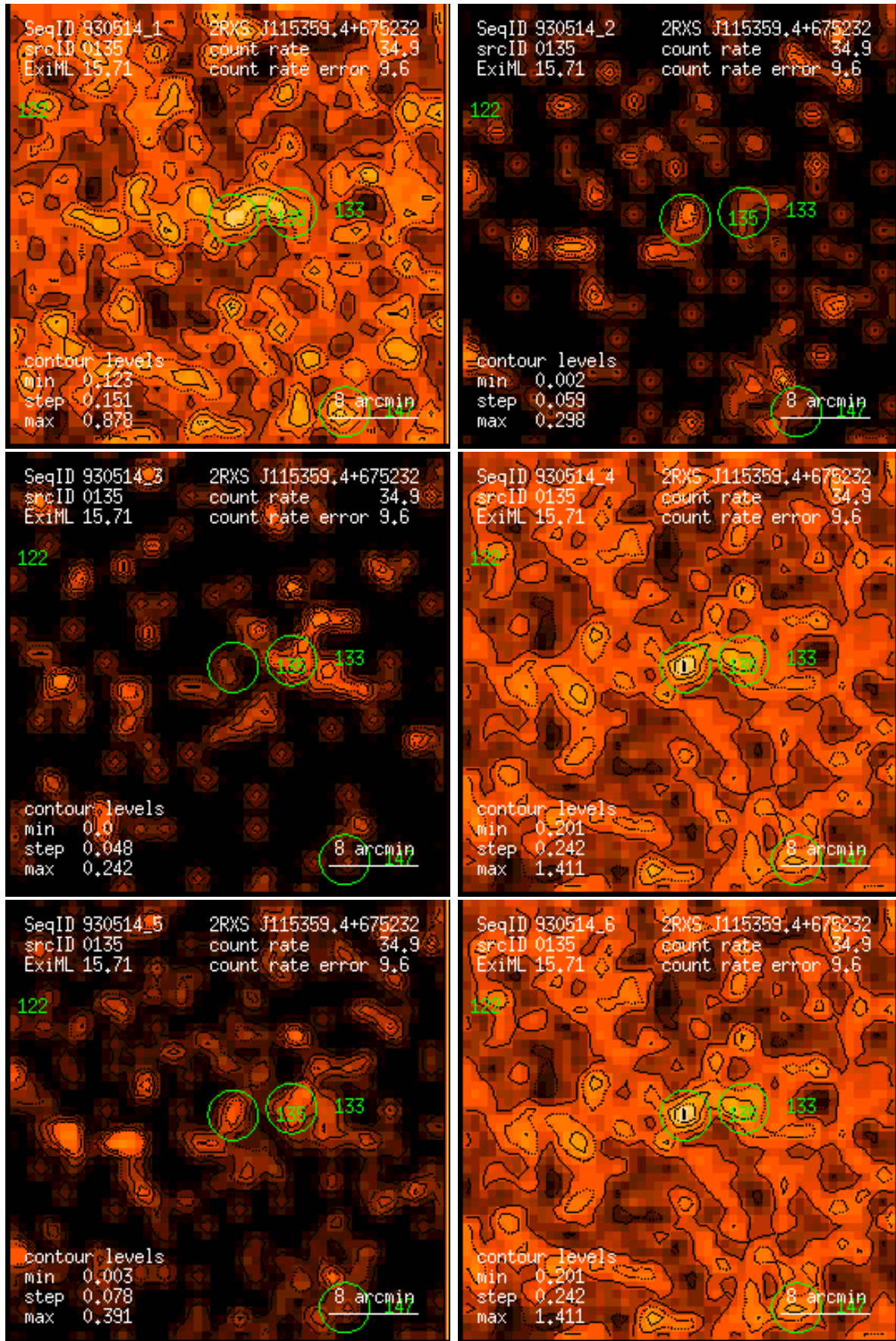
Figure 135: RASS 930514: detection 0135: band rate images, Gaussian filter: (1) PSPC channels 11 – 41, (2) 52 – 90, (3) 91 – 201, (4) 11 – 235, (5) 52 – 201, (6) 11 – 201. Broad band rates in counts/ks. Band rate contour levels in counts/ks/arcmin 2 .
