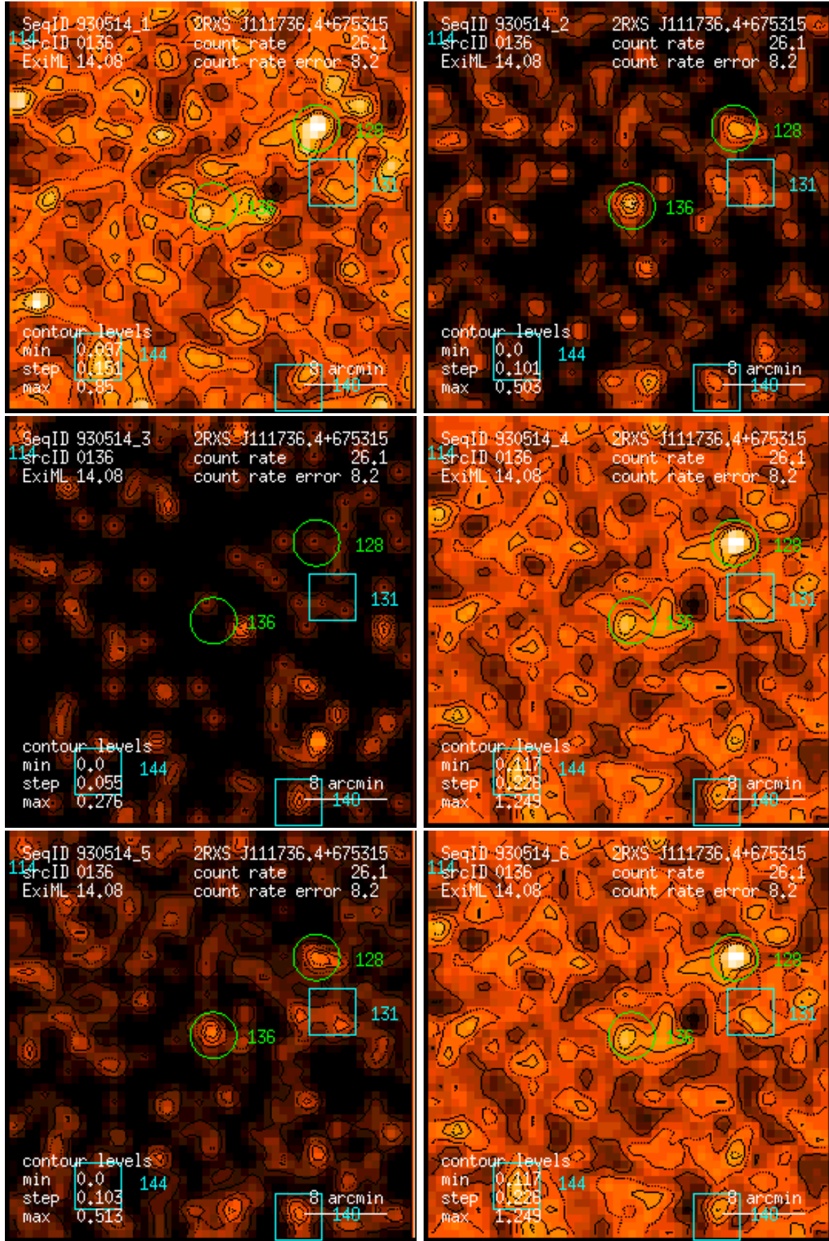
Figure 136: RASS 930514: detection 0136: band rate images, Gaussian filter: (1) PSPC channels 11 – 41, (2) 52 – 90, (3) 91 – 201, (4) 11 – 235, (5) 52 – 201, (6) 11 – 201. Broad band rates in counts/ks. Band rate contour levels in counts/ks/arcmin 2 .
