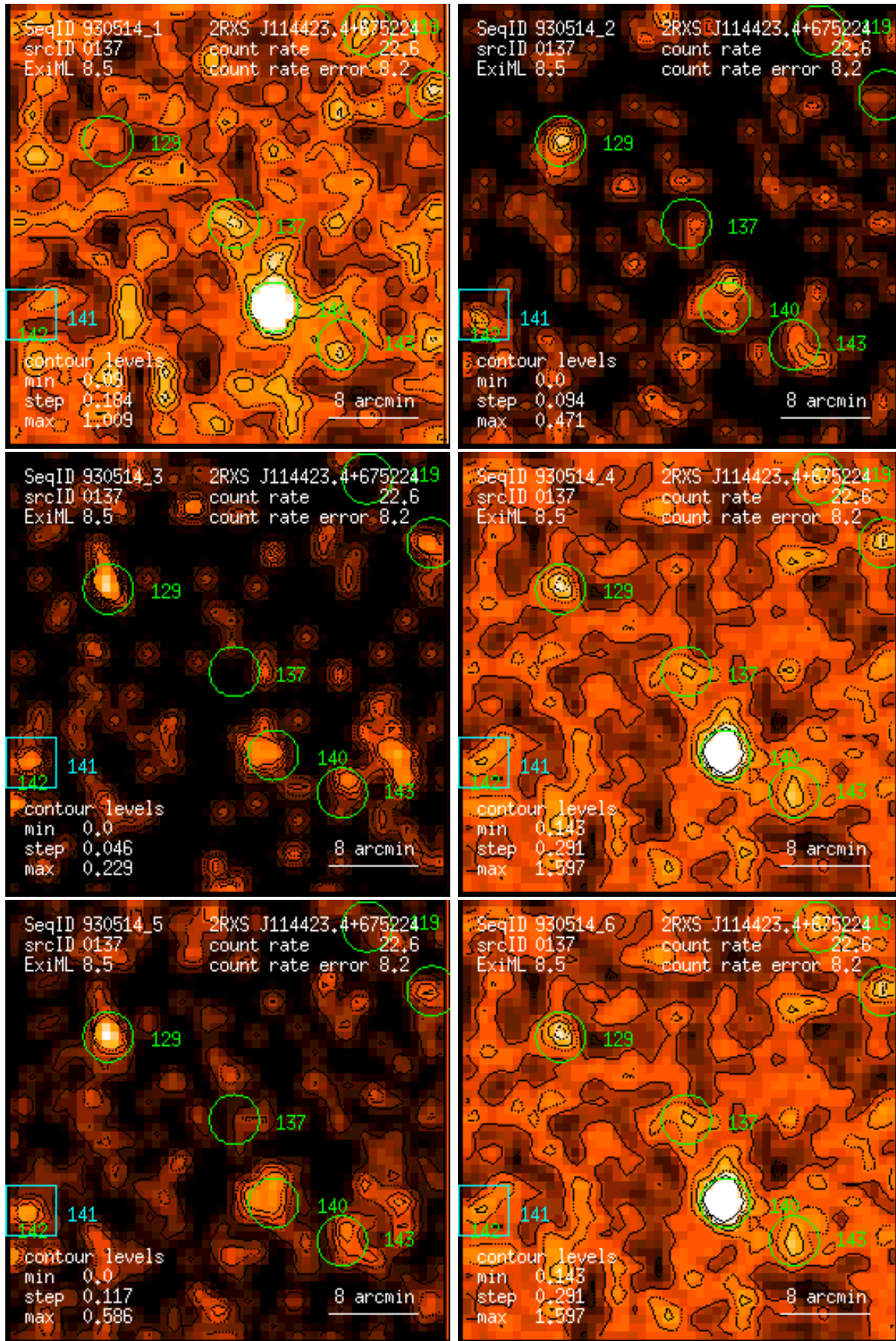
Figure 137: RASS 930514: detection 0137: band rate images, Gaussian filter: (1) PSPC channels 11 – 41, (2) 52 – 90, (3) 91 – 201, (4) 11 – 235, (5) 52 – 201, (6) 11 – 201. Broad band rates in counts/ks. Band rate contour levels in counts/ks/arcmin 2 .
