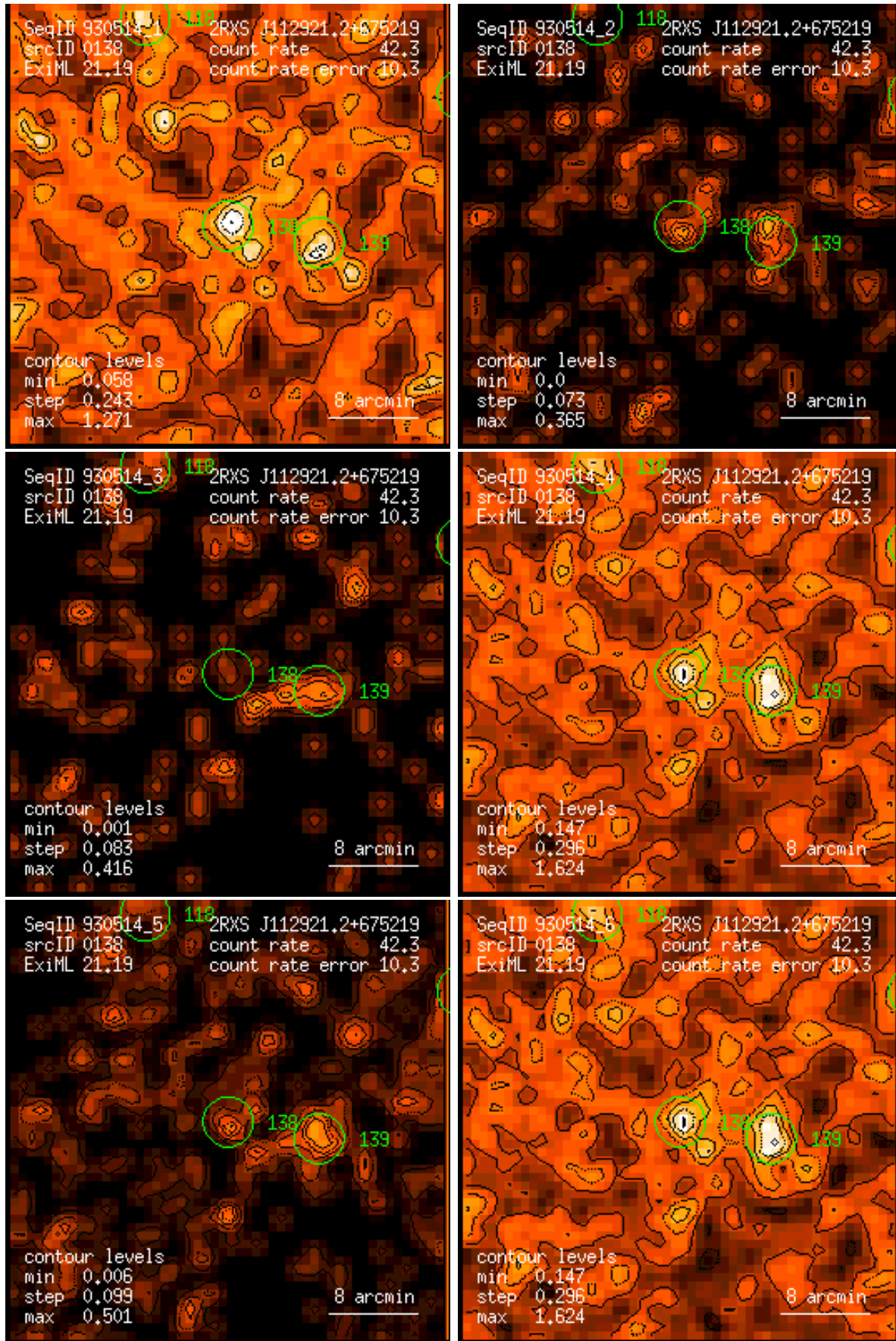
Figure 138: RASS 930514: detection 0138: band rate images, Gaussian filter: (1) PSPC channels 11 – 41, (2) 52 – 90, (3) 91 – 201, (4) 11 – 235, (5) 52 – 201, (6) 11 – 201. Broad band rates in counts/ks. Band rate contour levels in counts/ks/arcmin 2 .
