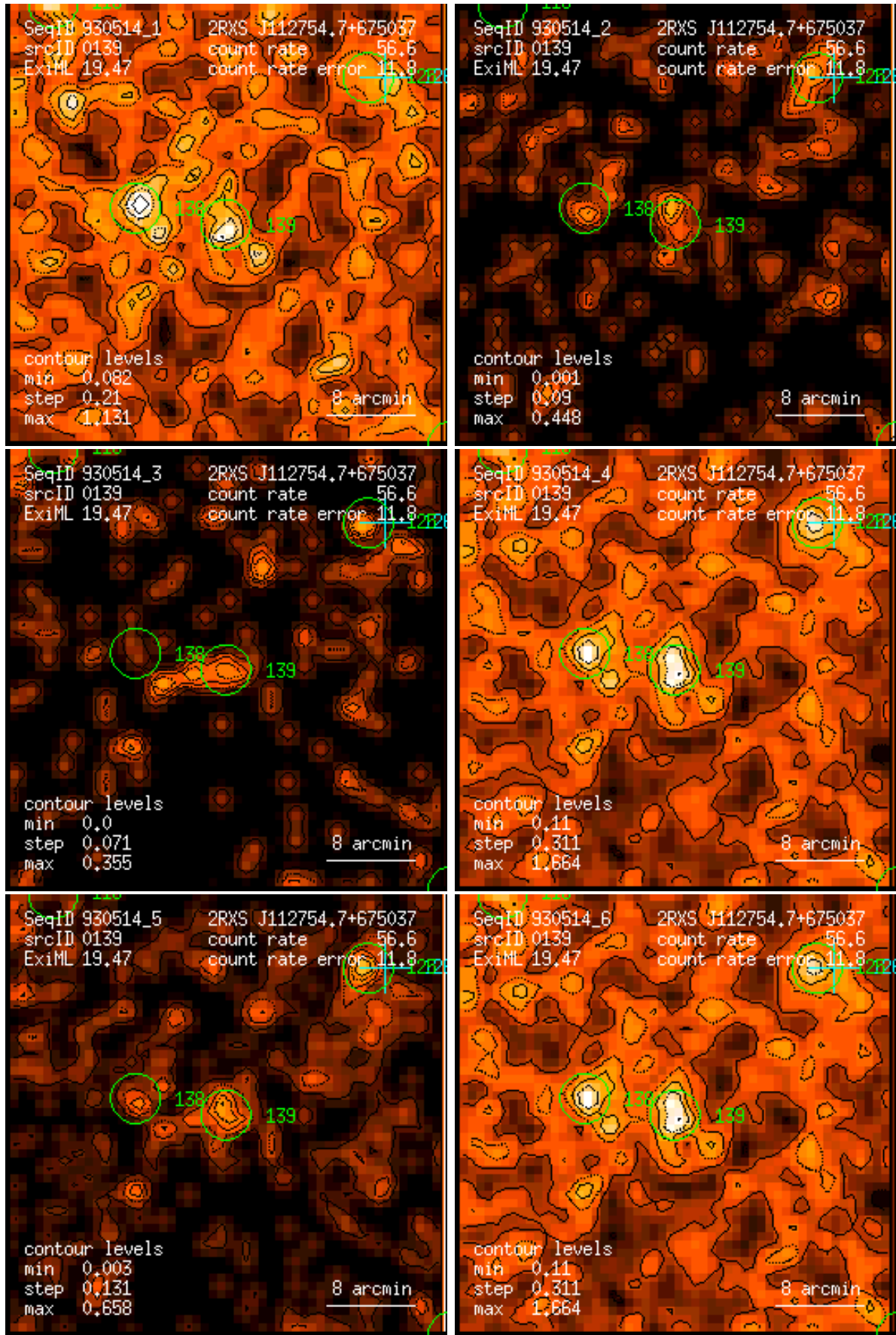
Figure 139: RASS 930514: detection 0139: band rate images, Gaussian filter: (1) PSPC channels 11 – 41, (2) 52 – 90, (3) 91 – 201, (4) 11 – 235, (5) 52 – 201, (6) 11 – 201. Broad band rates in counts/ks. Band rate contour levels in counts/ks/arcmin 2 .
