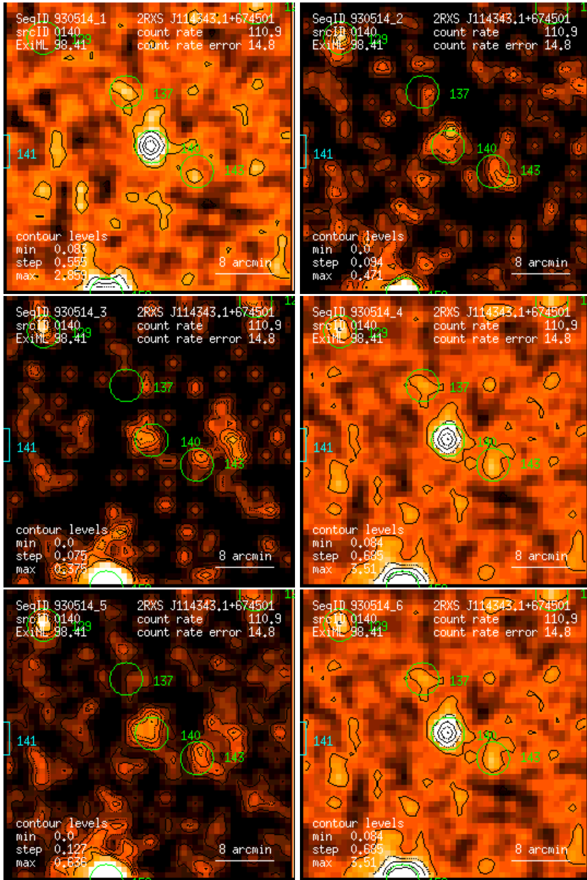
Figure 140: RASS 930514: detection 0140: band rate images, Gaussian filter: (1) PSPC channels 11 – 41, (2) 52 – 90, (3) 91 – 201, (4) 11 – 235, (5) 52 – 201, (6) 11 – 201. Broad band rates in counts/ks. Band rate contour levels in counts/ks/arcmin 2 .
