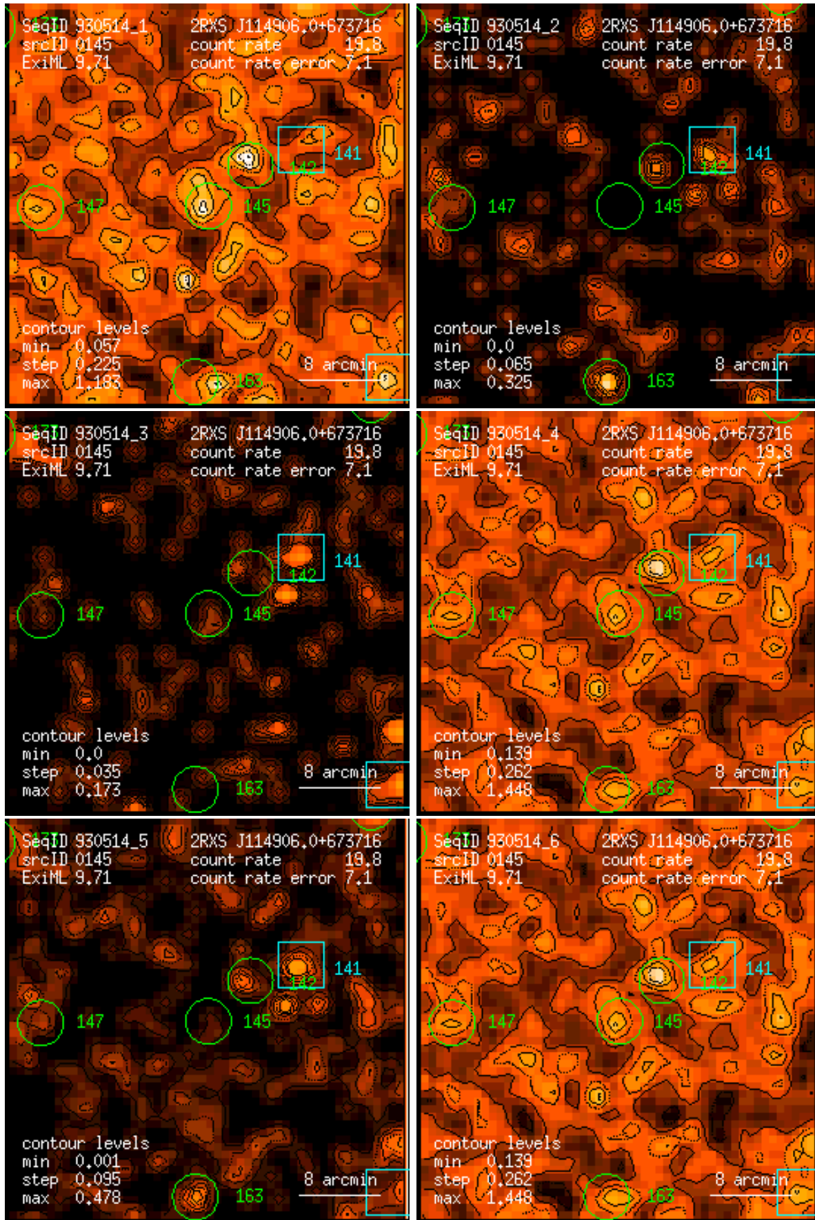
Figure 145: RASS 930514: detection 0145: band rate images, Gaussian filter: (1) PSPC channels 11 – 41, (2) 52 – 90, (3) 91 – 201, (4) 11 – 235, (5) 52 – 201, (6) 11 – 201. Broad band rates in counts/ks. Band rate contour levels in counts/ks/arcmin 2 .
