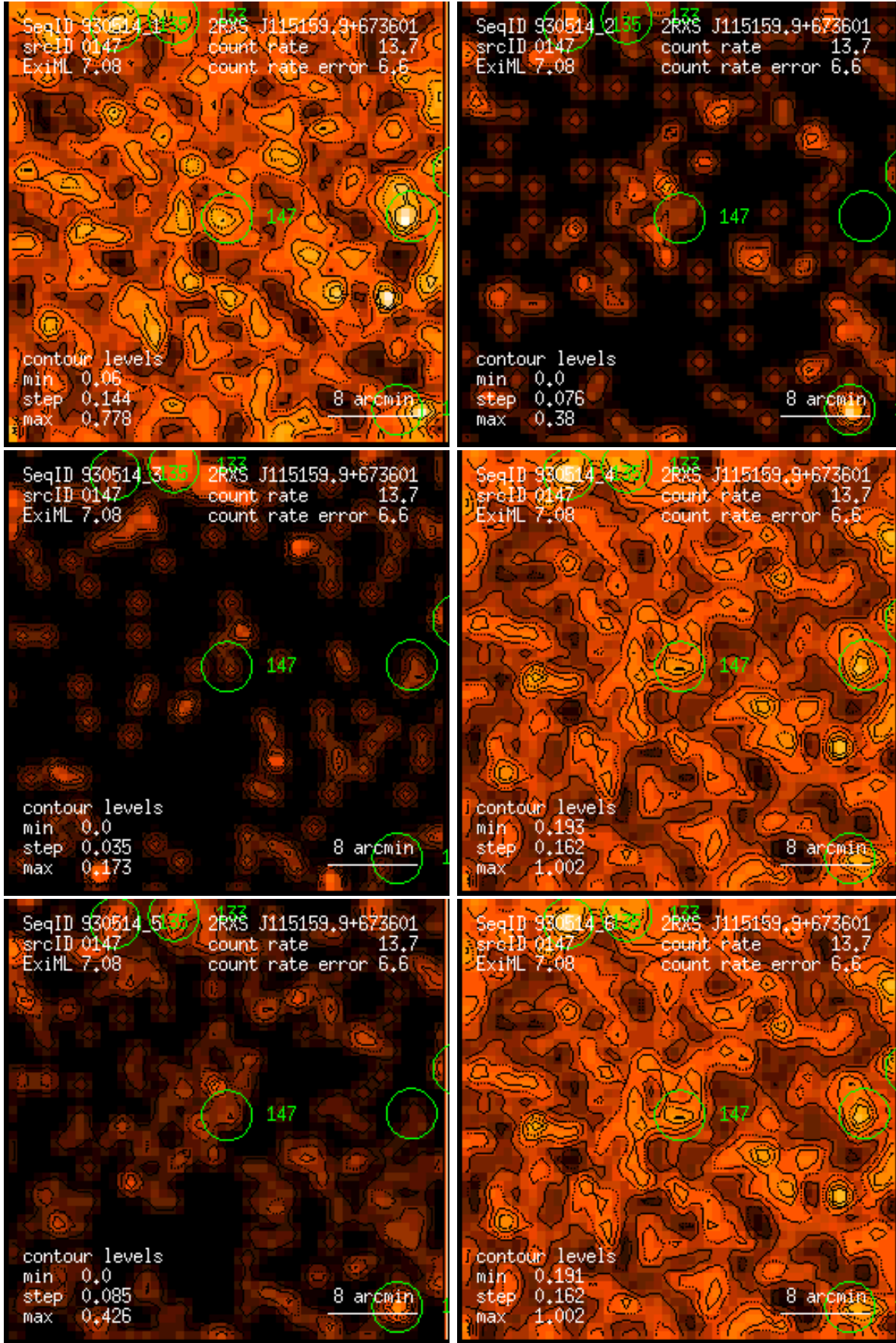
Figure 147: RASS 930514: detection 0147: band rate images, Gaussian filter: (1) PSPC channels 11 – 41, (2) 52 – 90, (3) 91 – 201, (4) 11 – 235, (5) 52 – 201, (6) 11 – 201. Broad band rates in counts/ks. Band rate contour levels in counts/ks/arcmin 2 .
