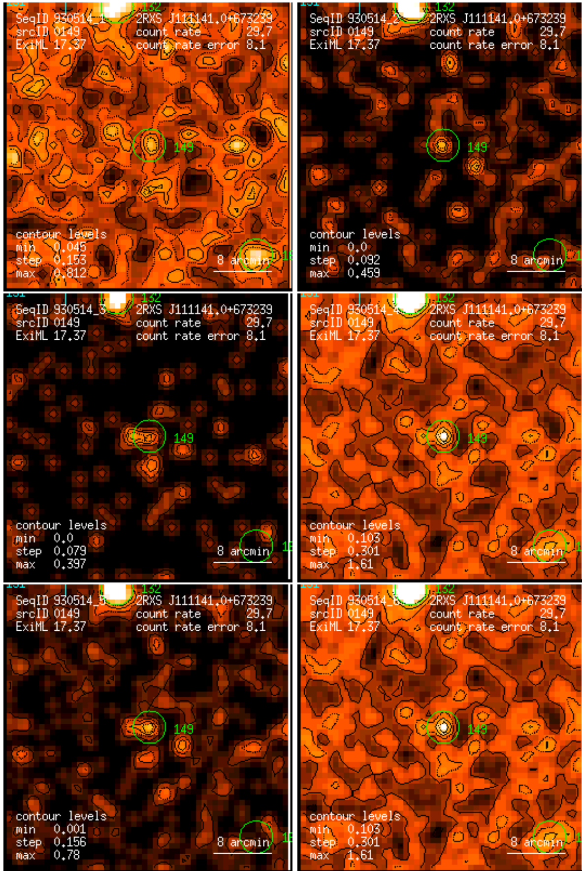
Figure 149: RASS 930514: detection 0149: band rate images, Gaussian filter: (1) PSPC channels 11 – 41, (2) 52 – 90, (3) 91 – 201, (4) 11 – 235, (5) 52 – 201, (6) 11 – 201. Broad band rates in counts/ks. Band rate contour levels in counts/ks/arcmin 2 .
