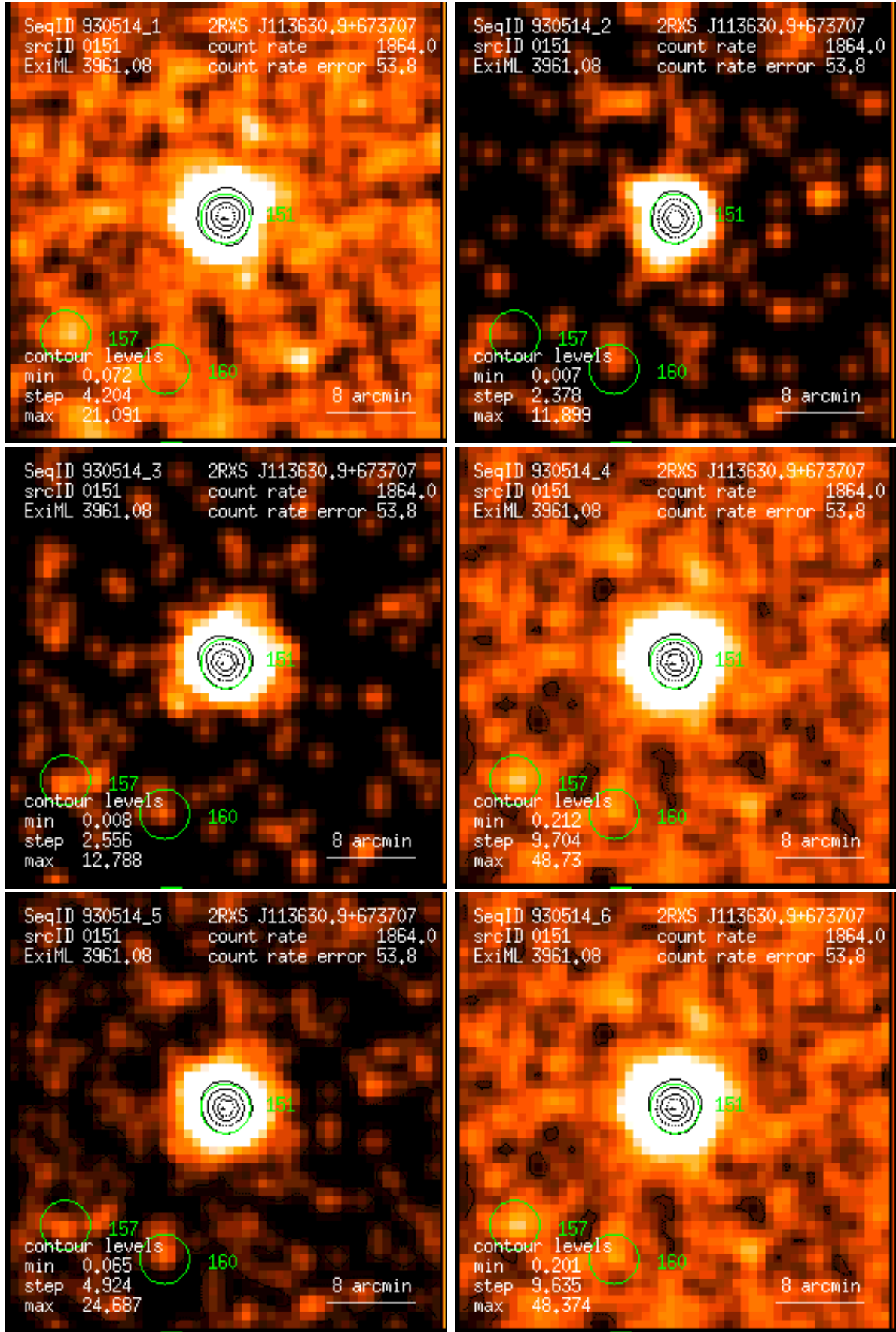
Figure 151: RASS 930514: detection 0151: band rate images, Gaussian filter: (1) PSPC channels 11 – 41, (2) 52 – 90, (3) 91 – 201, (4) 11 – 235, (5) 52 – 201, (6) 11 – 201. Broad band rates in counts/ks. Band rate contour levels in counts/ks/arcmin 2 .
