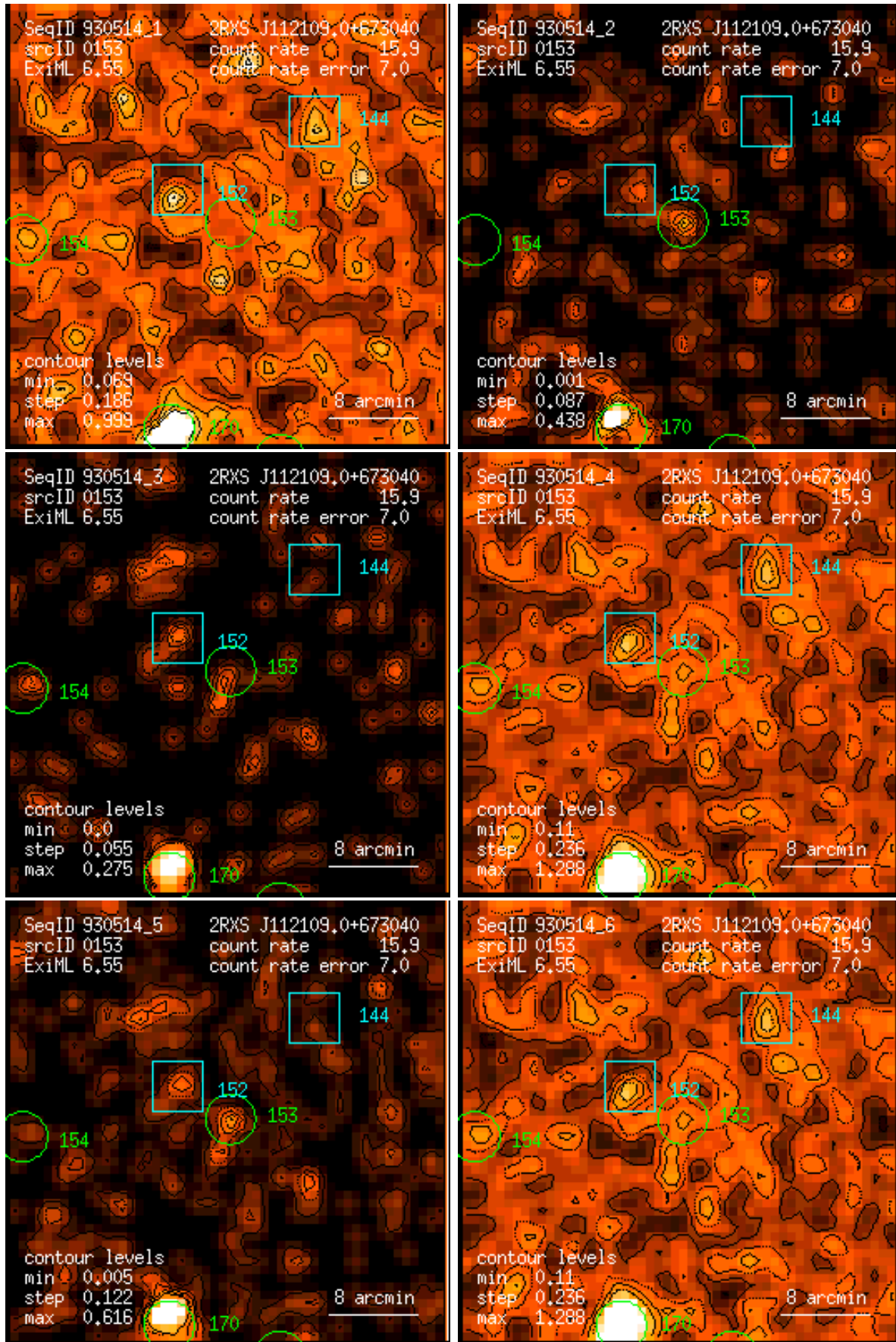
Figure 153: RASS 930514: detection 0153: band rate images, Gaussian filter: (1) PSPC channels 11 – 41, (2) 52 – 90, (3) 91 – 201, (4) 11 – 235, (5) 52 – 201, (6) 11 – 201. Broad band rates in counts/ks. Band rate contour levels in counts/ks/arcmin 2 .
