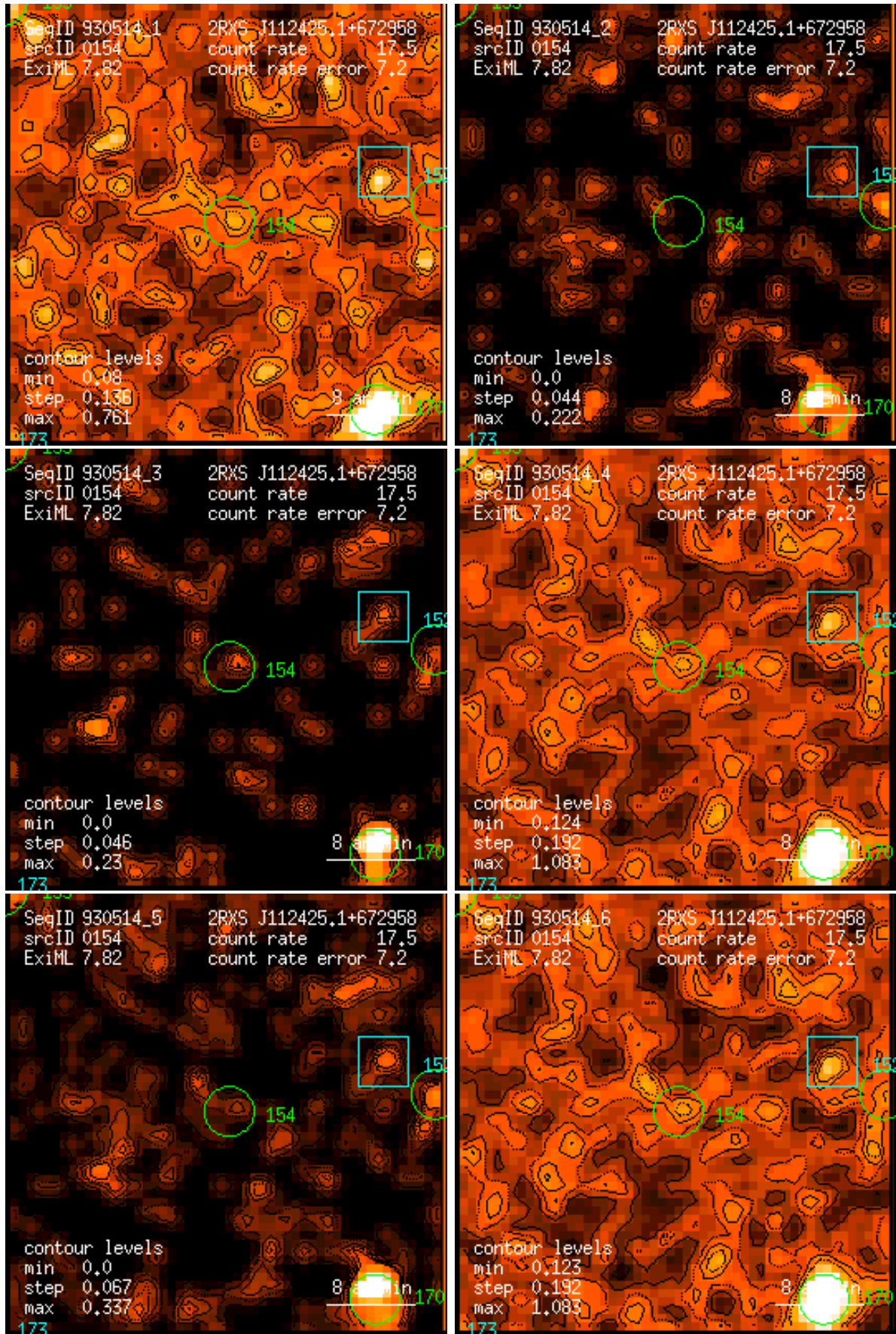
Figure 154: RASS 930514: detection 0154: band rate images, Gaussian filter: (1) PSPC channels 11 – 41, (2) 52 – 90, (3) 91 – 201, (4) 11 – 235, (5) 52 – 201, (6) 11 – 201. Broad band rates in counts/ks. Band rate contour levels in counts/ks/arcmin 2 .
