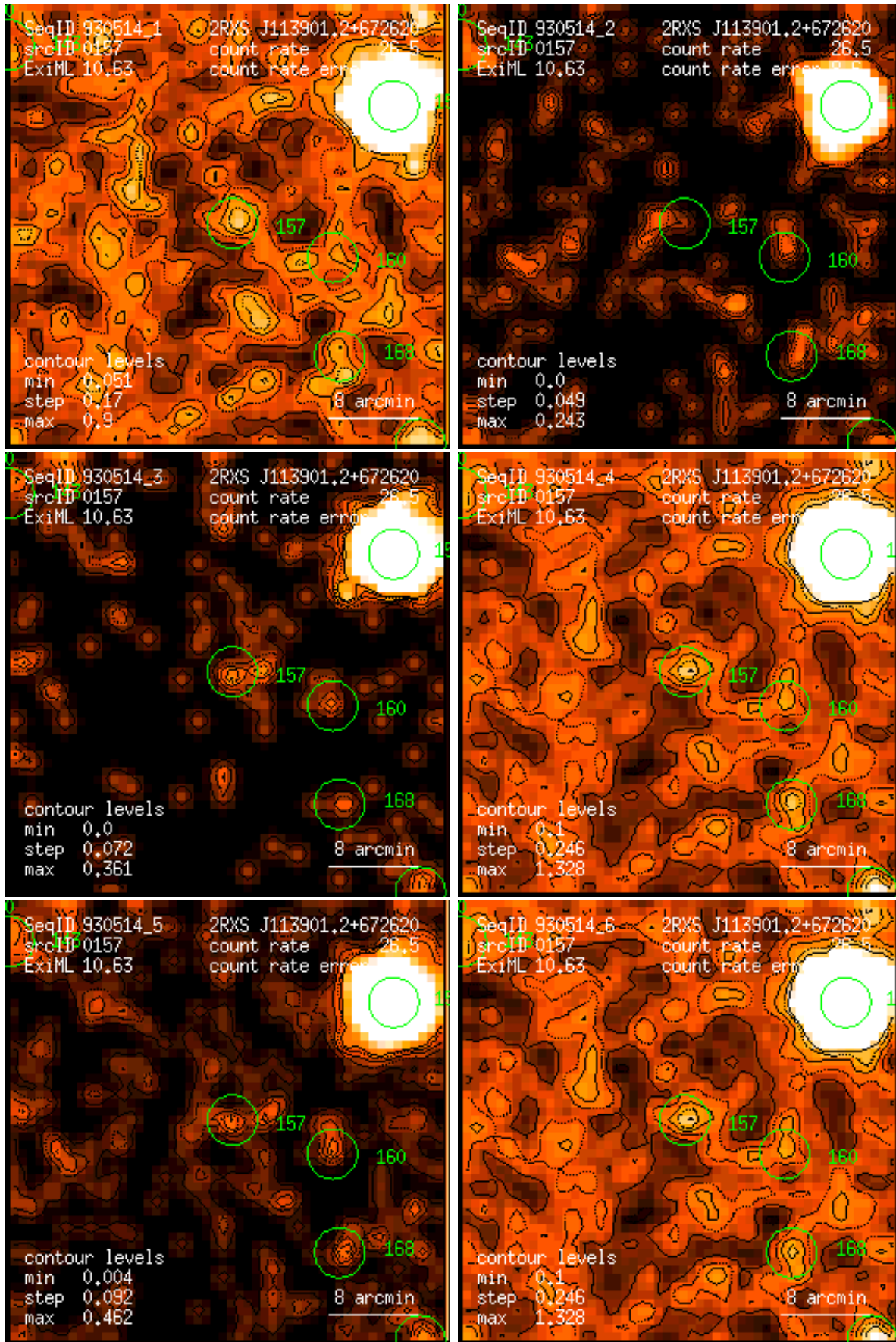
Figure 157: RASS 930514: detection 0157: band rate images, Gaussian filter: (1) PSPC channels 11 – 41, (2) 52 – 90, (3) 91 – 201, (4) 11 – 235, (5) 52 – 201, (6) 11 – 201. Broad band rates in counts/ks. Band rate contour levels in counts/ks/arcmin 2 .
