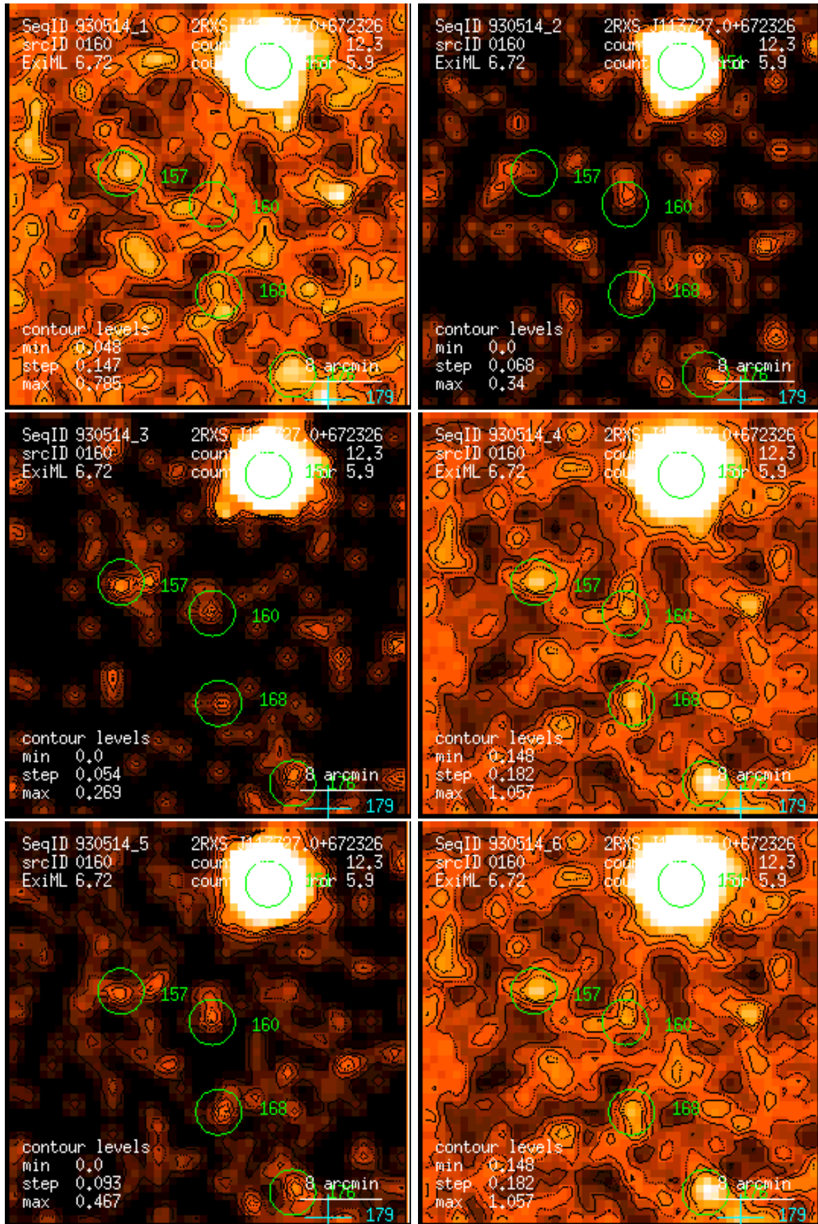
Figure 160: RASS 930514: detection 0160: band rate images, Gaussian filter: (1) PSPC channels 11 – 41, (2) 52 – 90, (3) 91 – 201, (4) 11 – 235, (5) 52 – 201, (6) 11 – 201. Broad band rates in counts/ks. Band rate contour levels in counts/ks/arcmin 2 .
