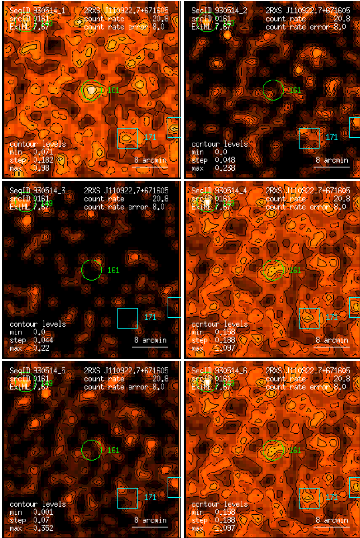
Figure 161: RASS 930514: detection 0161: band rate images, Gaussian filter: (1) PSPC channels 11 – 41, (2) 52 – 90, (3) 91 – 201, (4) 11 – 235, (5) 52 – 201, (6) 11 – 201. Broad band rates in counts/ks. Band rate contour levels in counts/ks/arcmin 2 .
