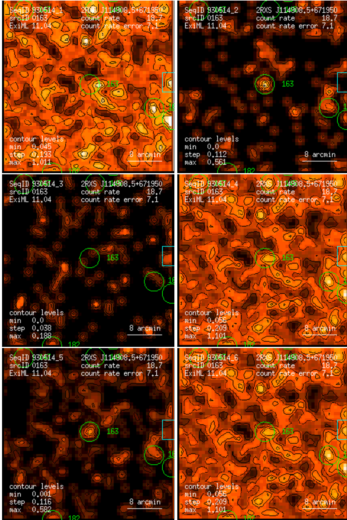
Figure 163: RASS 930514: detection 0163: band rate images, Gaussian filter: (1) PSPC channels 11 – 41, (2) 52 – 90, (3) 91 – 201, (4) 11 – 235, (5) 52 – 201, (6) 11 – 201. Broad band rates in counts/ks. Band rate contour levels in counts/ks/arcmin 2 .
