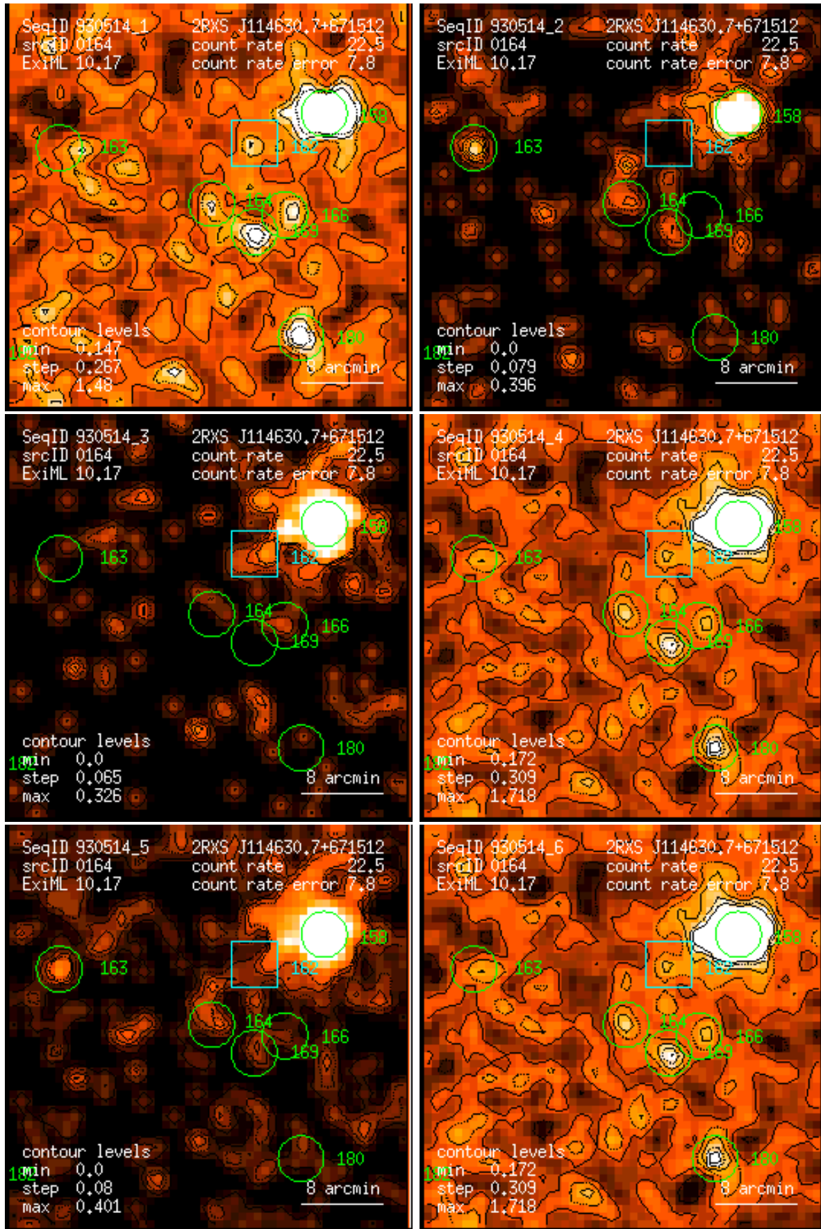
Figure 164: RASS 930514: detection 0164: band rate images, Gaussian filter: (1) PSPC channels 11 – 41, (2) 52 – 90, (3) 91 – 201, (4) 11 – 235, (5) 52 – 201, (6) 11 – 201. Broad band rates in counts/ks. Band rate contour levels in counts/ks/arcmin 2 .
