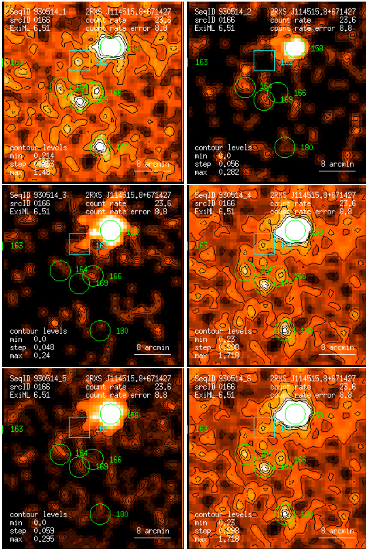
Figure 166: RASS 930514: detection 0166: band rate images, Gaussian filter: (1) PSPC channels 11 – 41, (2) 52 – 90, (3) 91 – 201, (4) 11 – 235, (5) 52 – 201, (6) 11 – 201. Broad band rates in counts/ks. Band rate contour levels in counts/ks/arcmin 2 .
