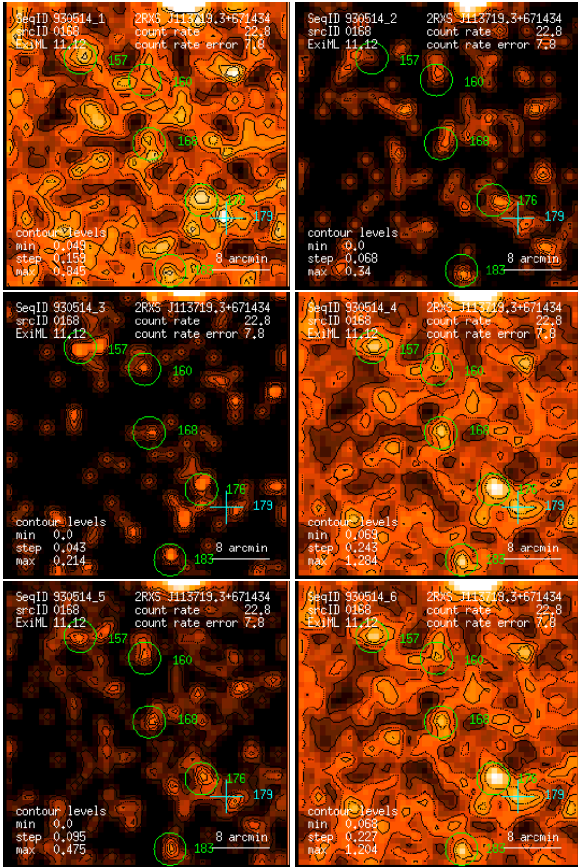
Figure 168: RASS 930514: detection 0168: band rate images, Gaussian filter: (1) PSPC channels 11 – 41, (2) 52 – 90, (3) 91 – 201, (4) 11 – 235, (5) 52 – 201, (6) 11 – 201. Broad band rates in counts/ks. Band rate contour levels in counts/ks/arcmin 2 .
