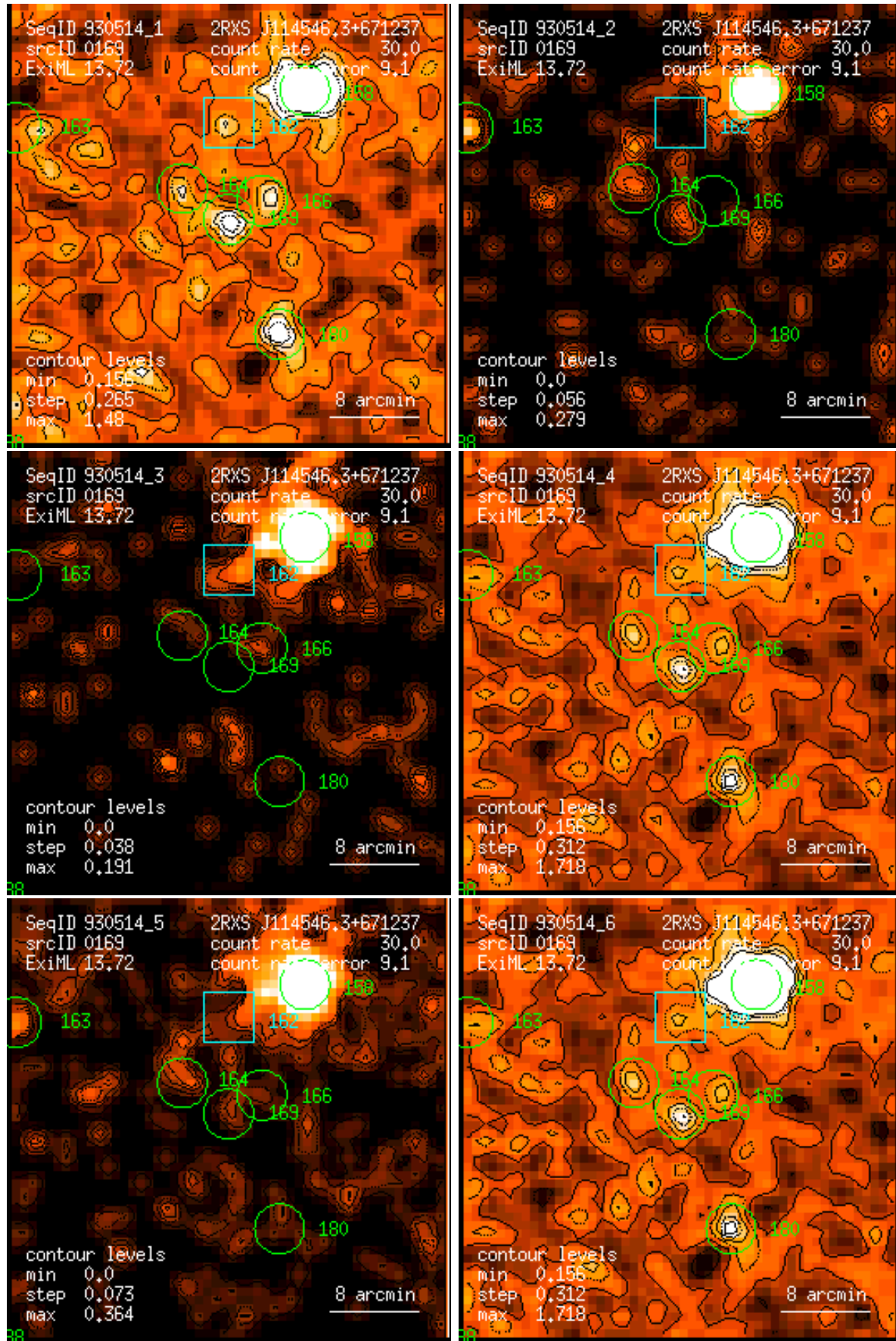
Figure 169: RASS 930514: detection 0169: band rate images, Gaussian filter: (1) PSPC channels 11 – 41, (2) 52 – 90, (3) 91 – 201, (4) 11 – 235, (5) 52 – 201, (6) 11 – 201. Broad band rates in counts/ks. Band rate contour levels in counts/ks/arcmin 2 .
