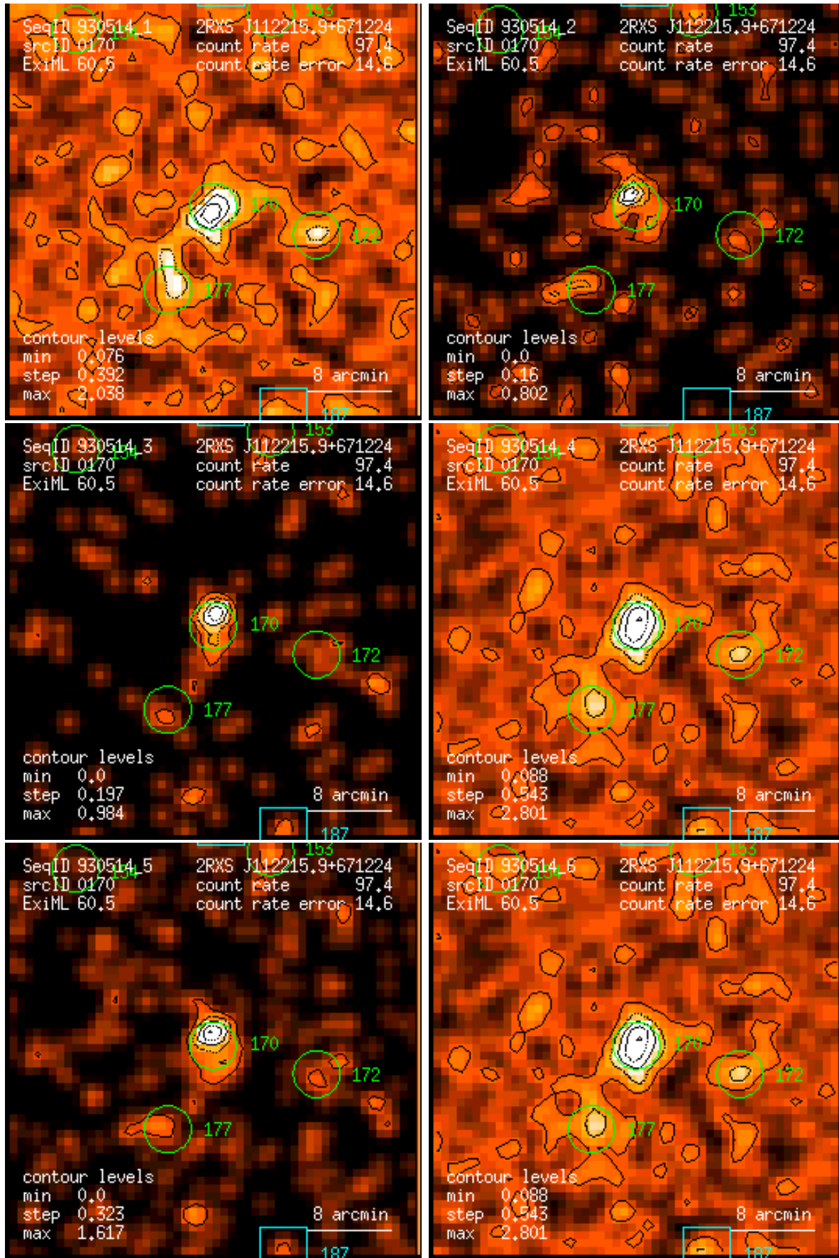
Figure 170: RASS 930514: detection 0170: band rate images, Gaussian filter: (1) PSPC channels 11 – 41, (2) 52 – 90, (3) 91 – 201, (4) 11 – 235, (5) 52 – 201, (6) 11 – 201. Broad band rates in counts/ks. Band rate contour levels in counts/ks/arcmin 2 .
