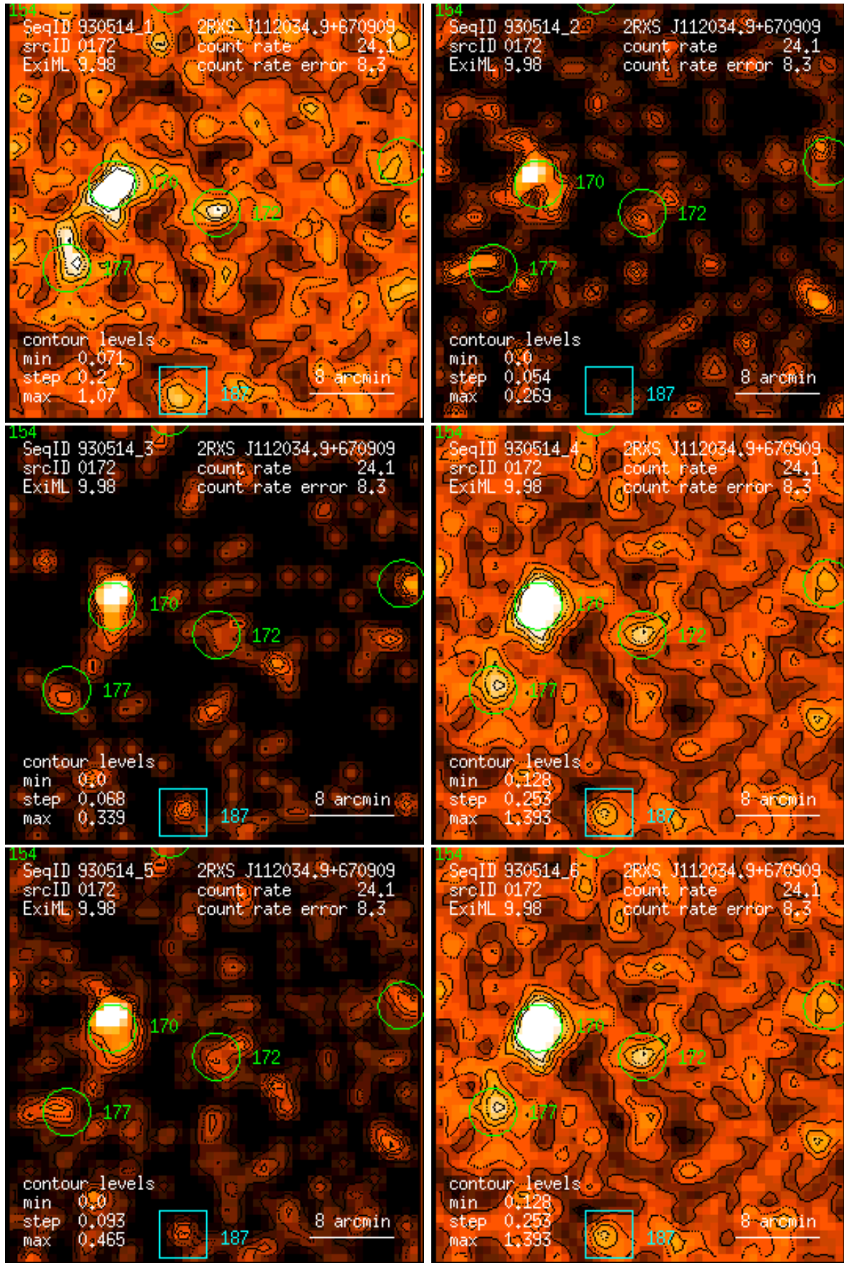
Figure 172: RASS 930514: detection 0172: band rate images, Gaussian filter: (1) PSPC channels 11 – 41, (2) 52 – 90, (3) 91 – 201, (4) 11 – 235, (5) 52 – 201, (6) 11 – 201. Broad band rates in counts/ks. Band rate contour levels in counts/ks/arcmin 2 .
