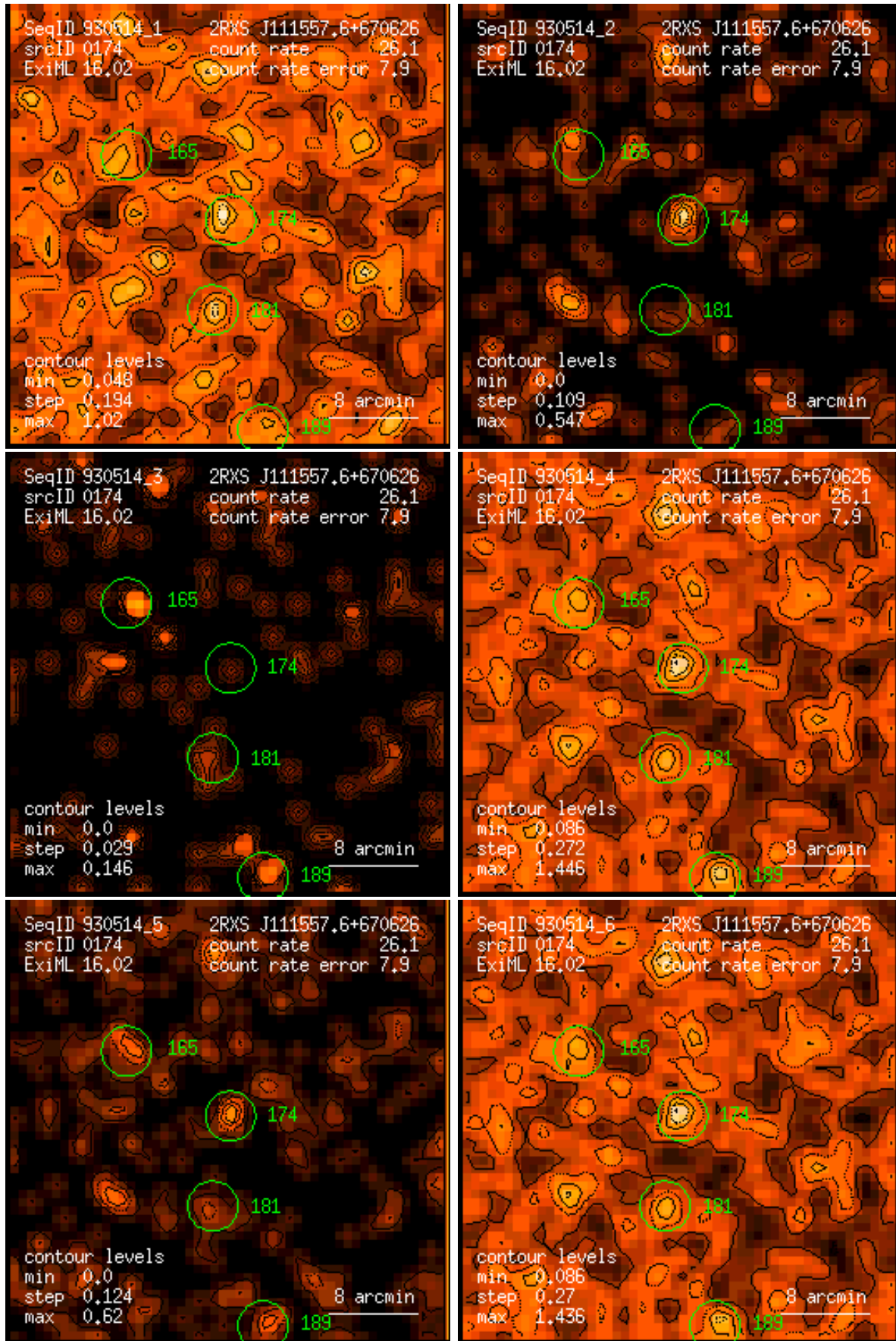
Figure 174: RASS 930514: detection 0174: band rate images, Gaussian filter: (1) PSPC channels 11 – 41, (2) 52 – 90, (3) 91 – 201, (4) 11 – 235, (5) 52 – 201, (6) 11 – 201. Broad band rates in counts/ks. Band rate contour levels in counts/ks/arcmin 2 .
