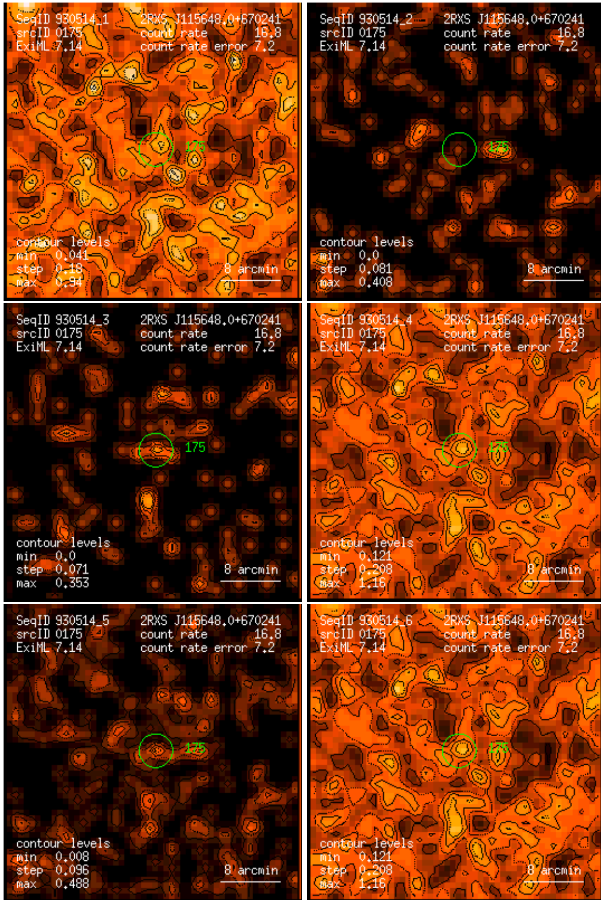
Figure 175: RASS 930514: detection 0175: band rate images, Gaussian filter: (1) PSPC channels 11 – 41, (2) 52 – 90, (3) 91 – 201, (4) 11 – 235, (5) 52 – 201, (6) 11 – 201. Broad band rates in counts/ks. Band rate contour levels in counts/ks/arcmin 2 .
