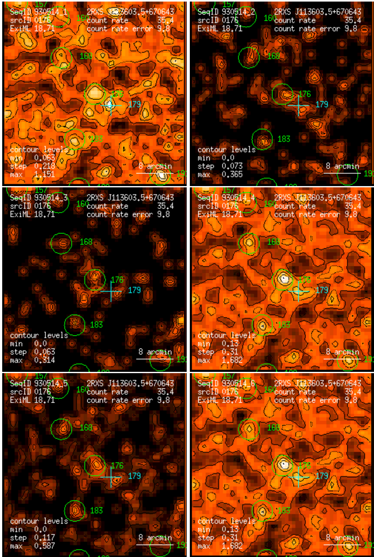
Figure 176: RASS 930514: detection 0176: band rate images, Gaussian filter: (1) PSPC channels 11 – 41, (2) 52 – 90, (3) 91 – 201, (4) 11 – 235, (5) 52 – 201, (6) 11 – 201. Broad band rates in counts/ks. Band rate contour levels in counts/ks/arcmin 2 .
