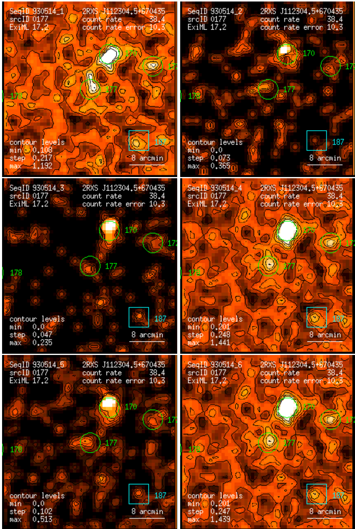
Figure 177: RASS 930514: detection 0177: band rate images, Gaussian filter: (1) PSPC channels 11 – 41, (2) 52 – 90, (3) 91 – 201, (4) 11 – 235, (5) 52 – 201, (6) 11 – 201. Broad band rates in counts/ks. Band rate contour levels in counts/ks/arcmin 2 .
