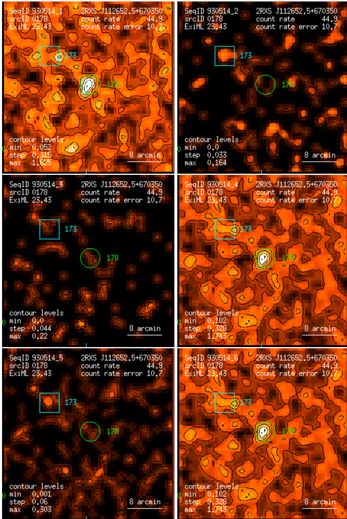
Figure 178: RASS 930514: detection 0178: band rate images, Gaussian filter: (1) PSPC channels 11 – 41, (2) 52 – 90, (3) 91 – 201, (4) 11 – 235, (5) 52 – 201, (6) 11 – 201. Broad band rates in counts/ks. Band rate contour levels in counts/ks/arcmin 2 .
