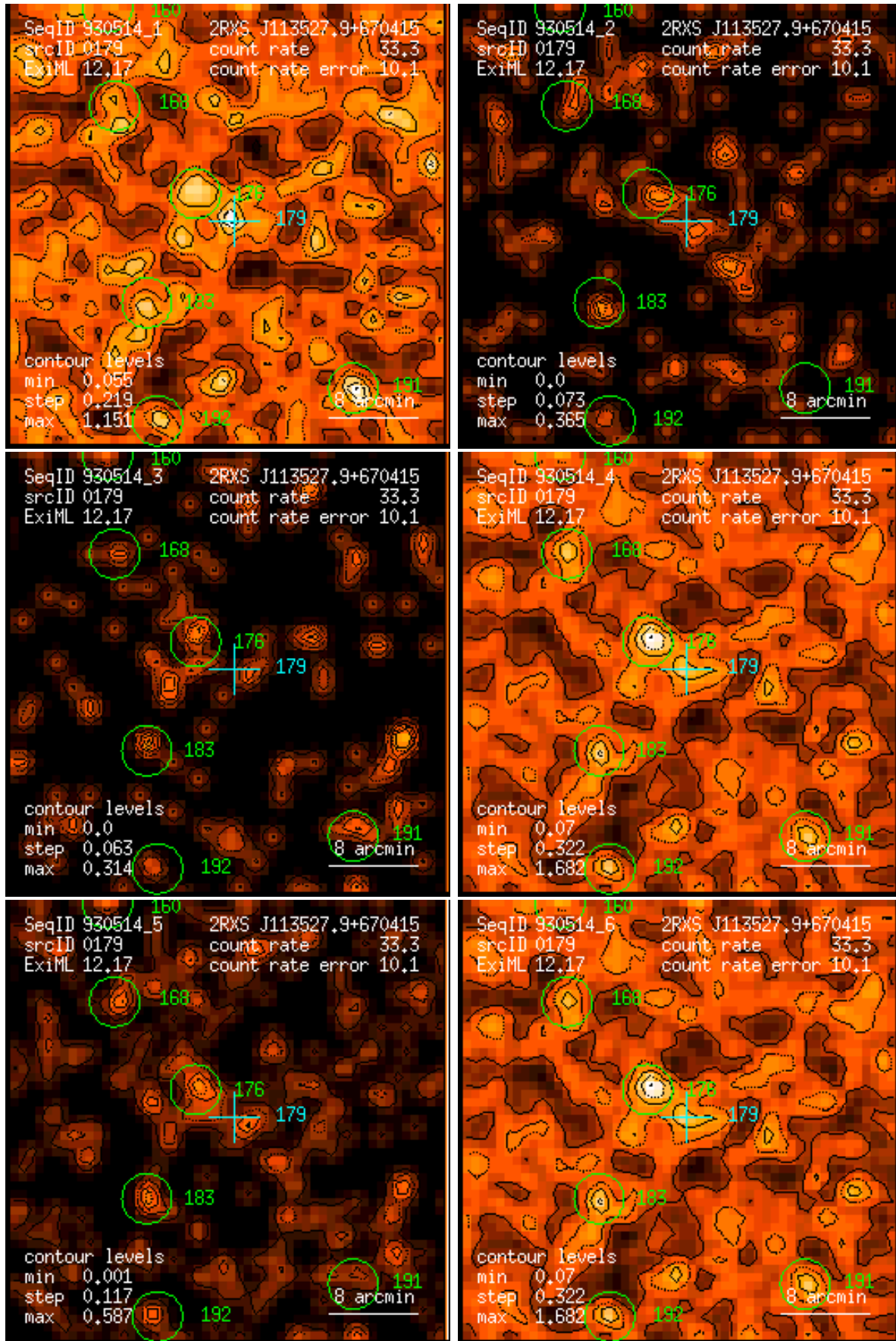
Figure 179: RASS 930514: detection 0179: band rate images, Gaussian filter: (1) PSPC channels 11 – 41, (2) 52 – 90, (3) 91 – 201, (4) 11 – 235, (5) 52 – 201, (6) 11 – 201. Broad band rates in counts/ks. Band rate contour levels in counts/ks/arcmin 2 .
