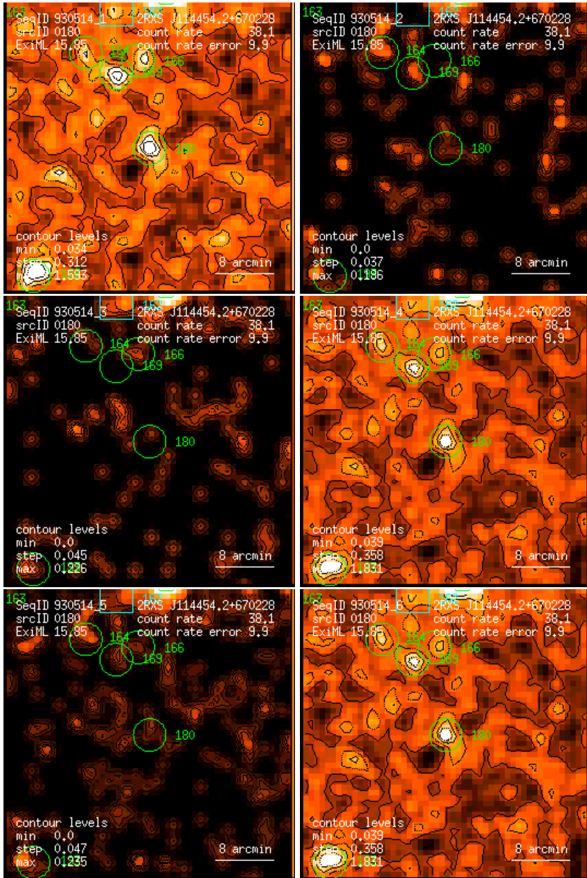
Figure 180: RASS 930514: detection 0180: band rate images, Gaussian filter: (1) PSPC channels 11 – 41, (2) 52 – 90, (3) 91 – 201, (4) 11 – 235, (5) 52 – 201, (6) 11 – 201. Broad band rates in counts/ks. Band rate contour levels in counts/ks/arcmin 2 .
