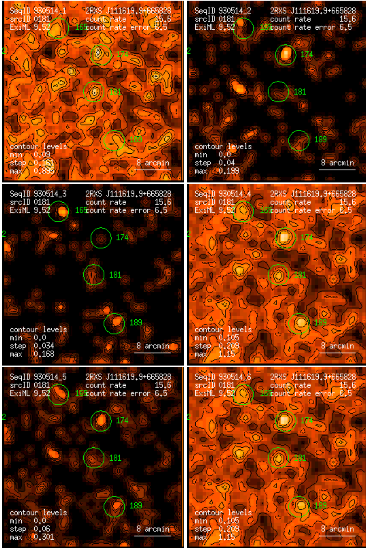
Figure 181: RASS 930514: detection 0181: band rate images, Gaussian filter: (1) PSPC channels 11 – 41, (2) 52 – 90, (3) 91 – 201, (4) 11 – 235, (5) 52 – 201, (6) 11 – 201. Broad band rates in counts/ks. Band rate contour levels in counts/ks/arcmin 2 .
