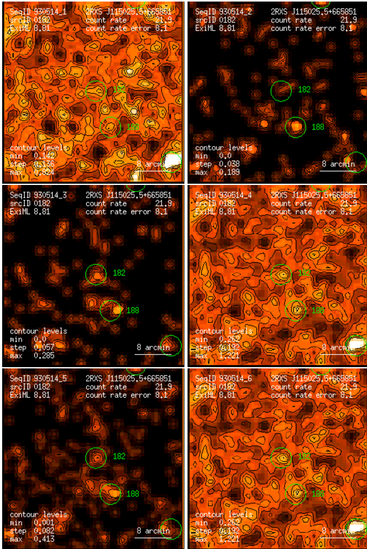
Figure 182: RASS 930514: detection 0182: band rate images, Gaussian filter: (1) PSPC channels 11 – 41, (2) 52 – 90, (3) 91 – 201, (4) 11 – 235, (5) 52 – 201, (6) 11 – 201. Broad band rates in counts/ks. Band rate contour levels in counts/ks/arcmin 2 .
