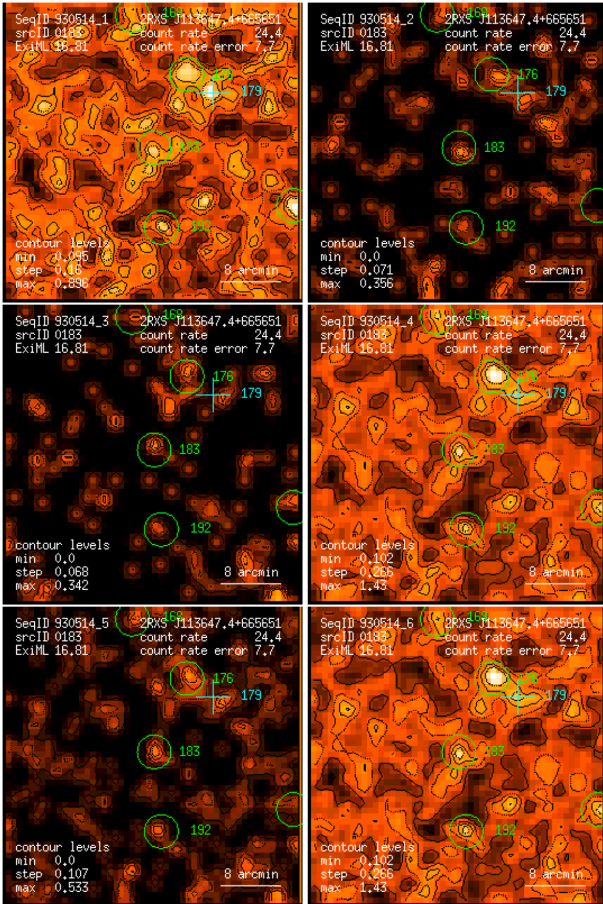
Figure 183: RASS 930514: detection 0183: band rate images, Gaussian filter: (1) PSPC channels 11 – 41, (2) 52 – 90, (3) 91 – 201, (4) 11 – 235, (5) 52 – 201, (6) 11 – 201. Broad band rates in counts/ks. Band rate contour levels in counts/ks/arcmin 2 .
