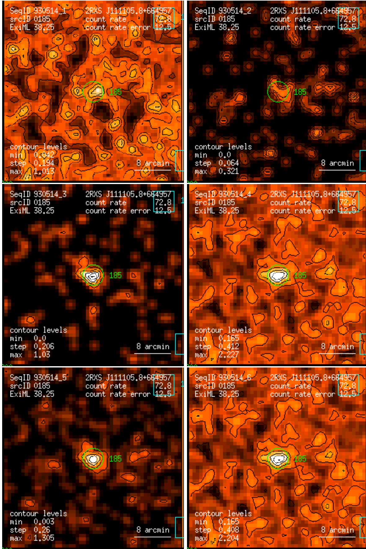
Figure 185: RASS 930514: detection 0185: band rate images, Gaussian filter: (1) PSPC channels 11 – 41, (2) 52 – 90, (3) 91 – 201, (4) 11 – 235, (5) 52 – 201, (6) 11 – 201. Broad band rates in counts/ks. Band rate contour levels in counts/ks/arcmin 2 .
