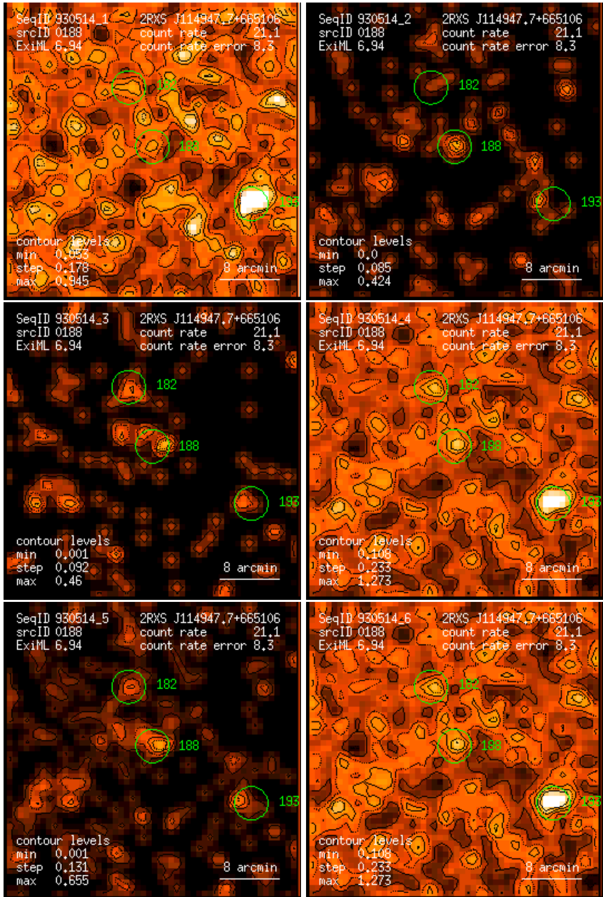
Figure 188: RASS 930514: detection 0188: band rate images, Gaussian filter: (1) PSPC channels 11 – 41, (2) 52 – 90, (3) 91 – 201, (4) 11 – 235, (5) 52 – 201, (6) 11 – 201. Broad band rates in counts/ks. Band rate contour levels in counts/ks/arcmin 2 .
