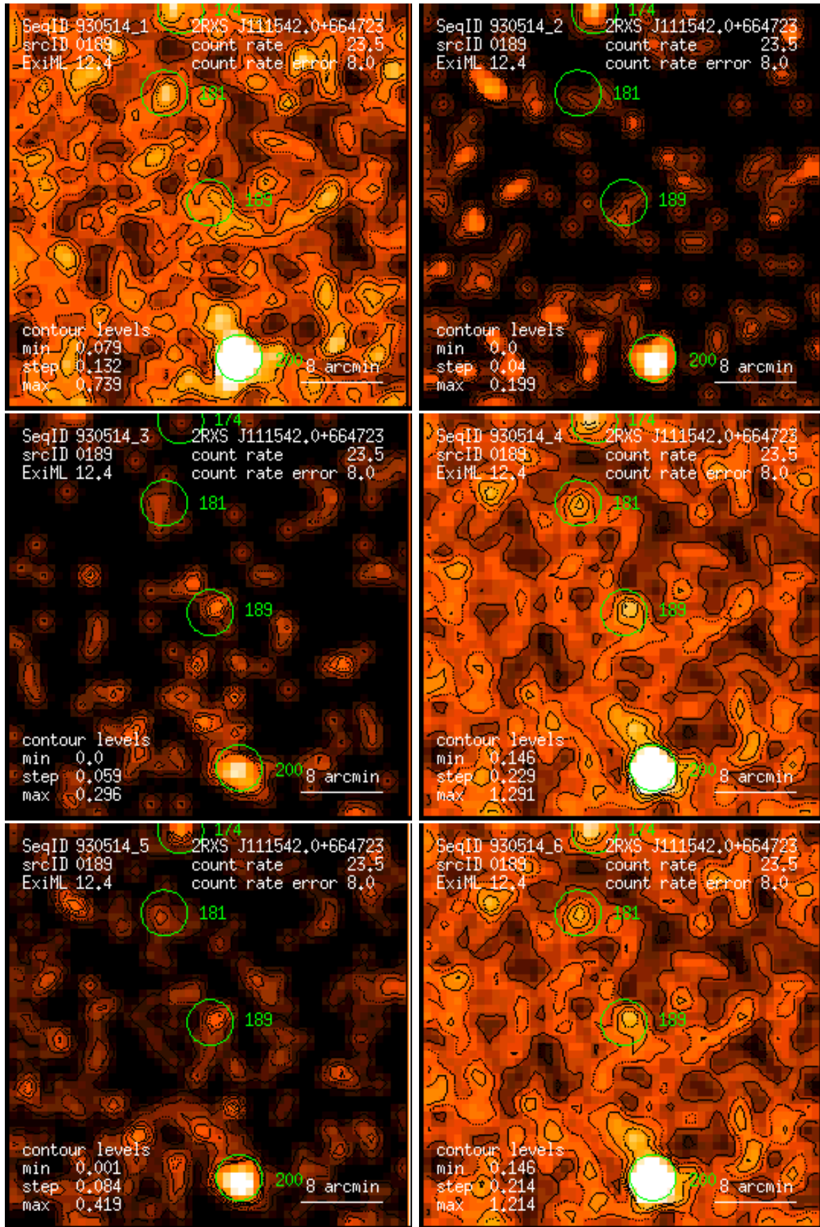
Figure 189: RASS 930514: detection 0189: band rate images, Gaussian filter: (1) PSPC channels 11 – 41, (2) 52 – 90, (3) 91 – 201, (4) 11 – 235, (5) 52 – 201, (6) 11 – 201. Broad band rates in counts/ks. Band rate contour levels in counts/ks/arcmin 2 .
