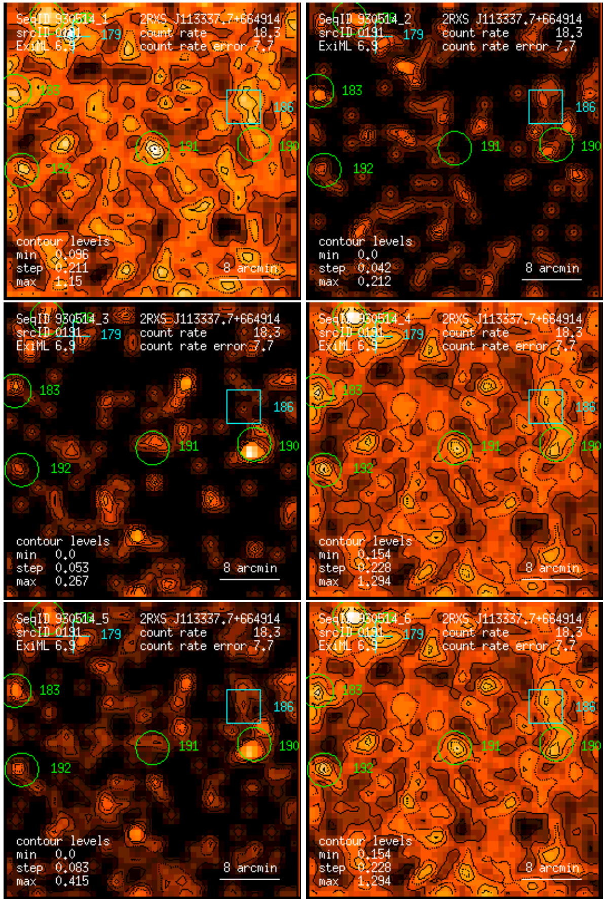
Figure 191: RASS 930514: detection 0191: band rate images, Gaussian filter: (1) PSPC channels 11 – 41, (2) 52 – 90, (3) 91 – 201, (4) 11 – 235, (5) 52 – 201, (6) 11 – 201. Broad band rates in counts/ks. Band rate contour levels in counts/ks/arcmin 2 .
