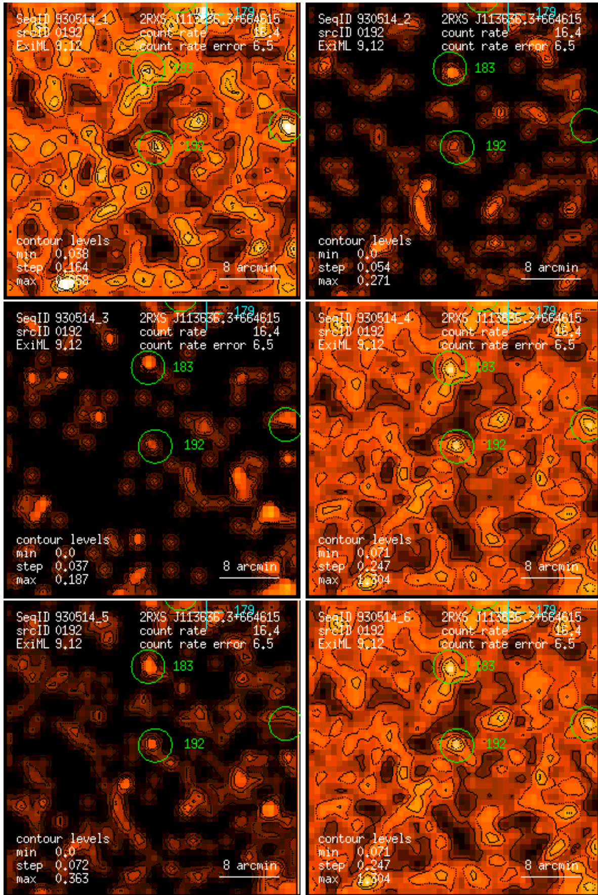
Figure 192: RASS 930514: detection 0192: band rate images, Gaussian filter: (1) PSPC channels 11 – 41, (2) 52 – 90, (3) 91 – 201, (4) 11 – 235, (5) 52 – 201, (6) 11 – 201. Broad band rates in counts/ks. Band rate contour levels in counts/ks/arcmin 2 .
